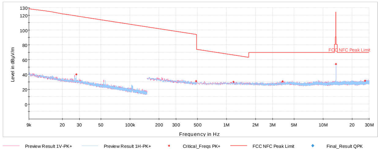
Plot 7-8. Radiated Spurious Plot 9kHz – 30MHz (CE A 848kbps)
