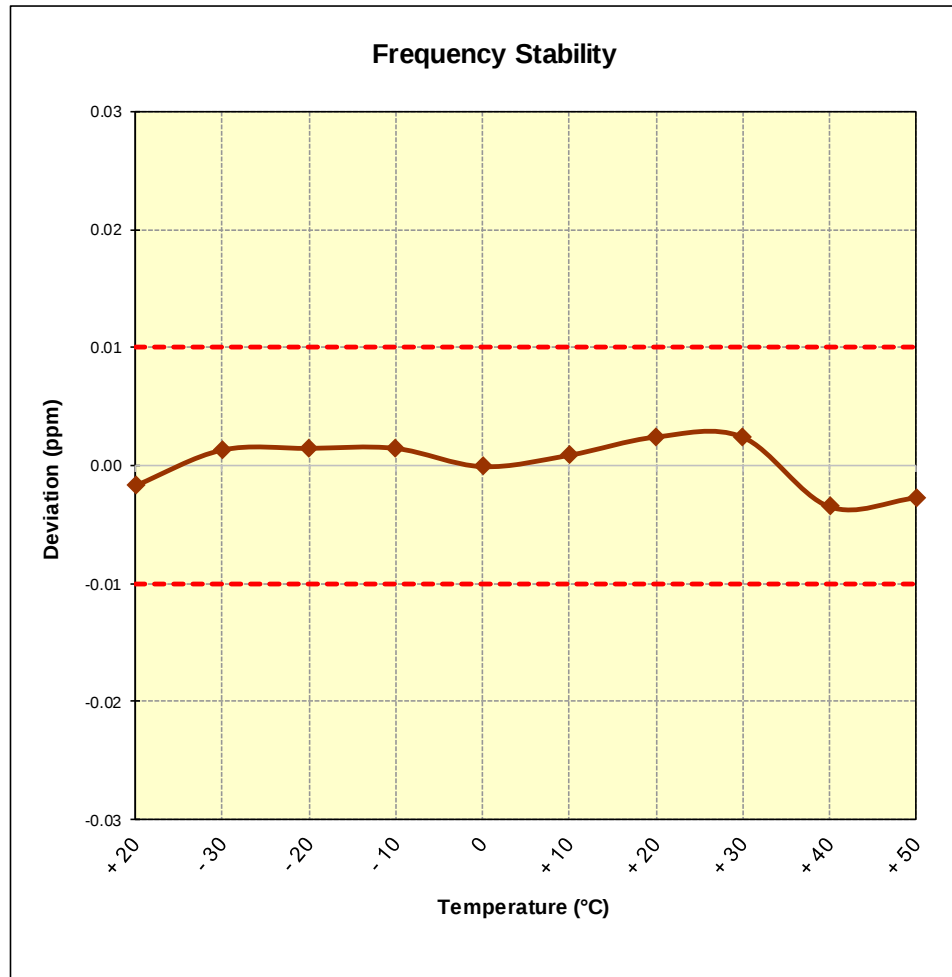
Figure 7-2. Frequency Stability Plot (CE A 848kbps)
