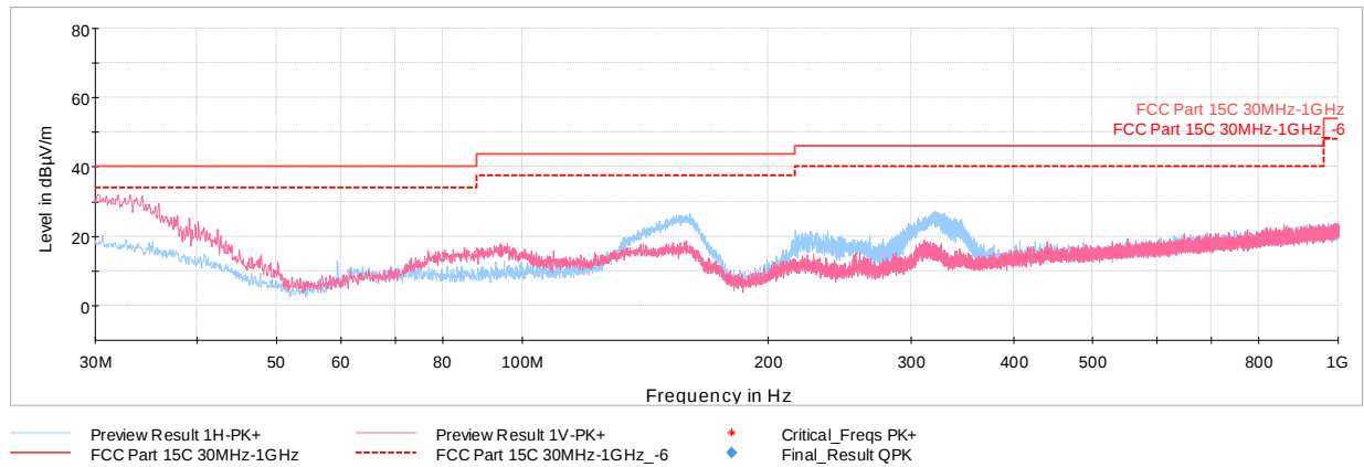
Plot 7-11. Radiated Spurious Plot 30MHz – 1GHz (Reader 10% Ask 1 out of 256, with WCP + AC/DC Adapter)
