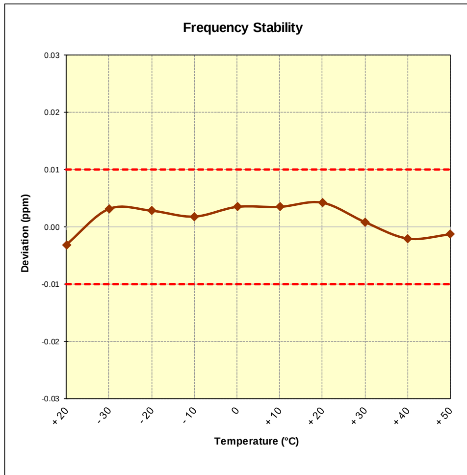
Figure 7-3. Frequency Stability Plot (Reader 10% Ask 1 out of 256)
