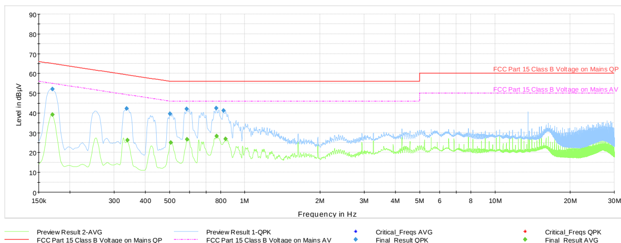
Plot 7-12. Line-Conducted Test Plot (L1, with WCP + AC/DC Adapter attached)
