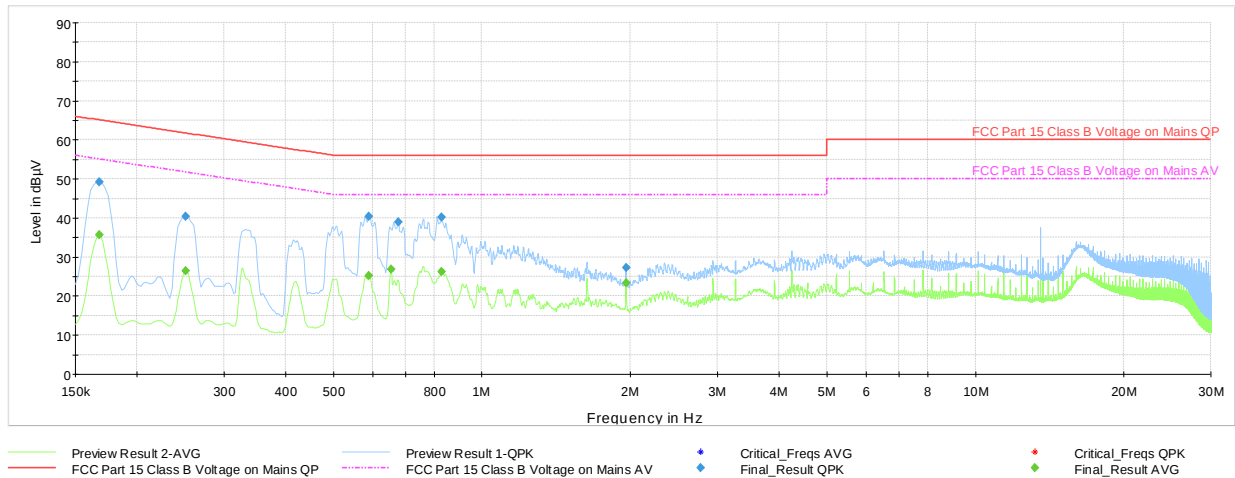
Plot 7-13. Line-Conducted Test Plot (N, with WCP + AC/DC Adapter attached)
