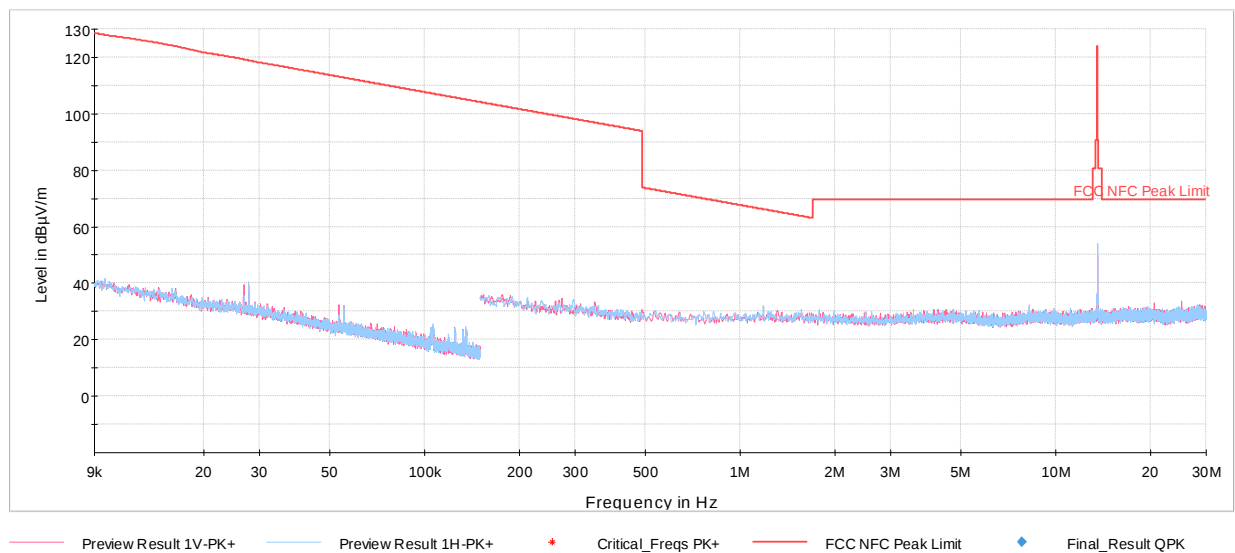
Plot 7-9. Radiated Spurious Plot 9kHz – 30MHz (Reader 10% Ask 1 out of 256)
