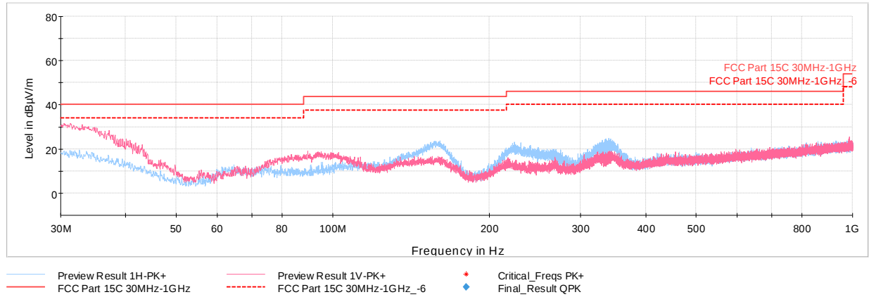
Plot 7-10. Radiated Spurious Plot 30MHz – 1GHz (CE A 848kbps, with WCP + AC/DC Adapter)
