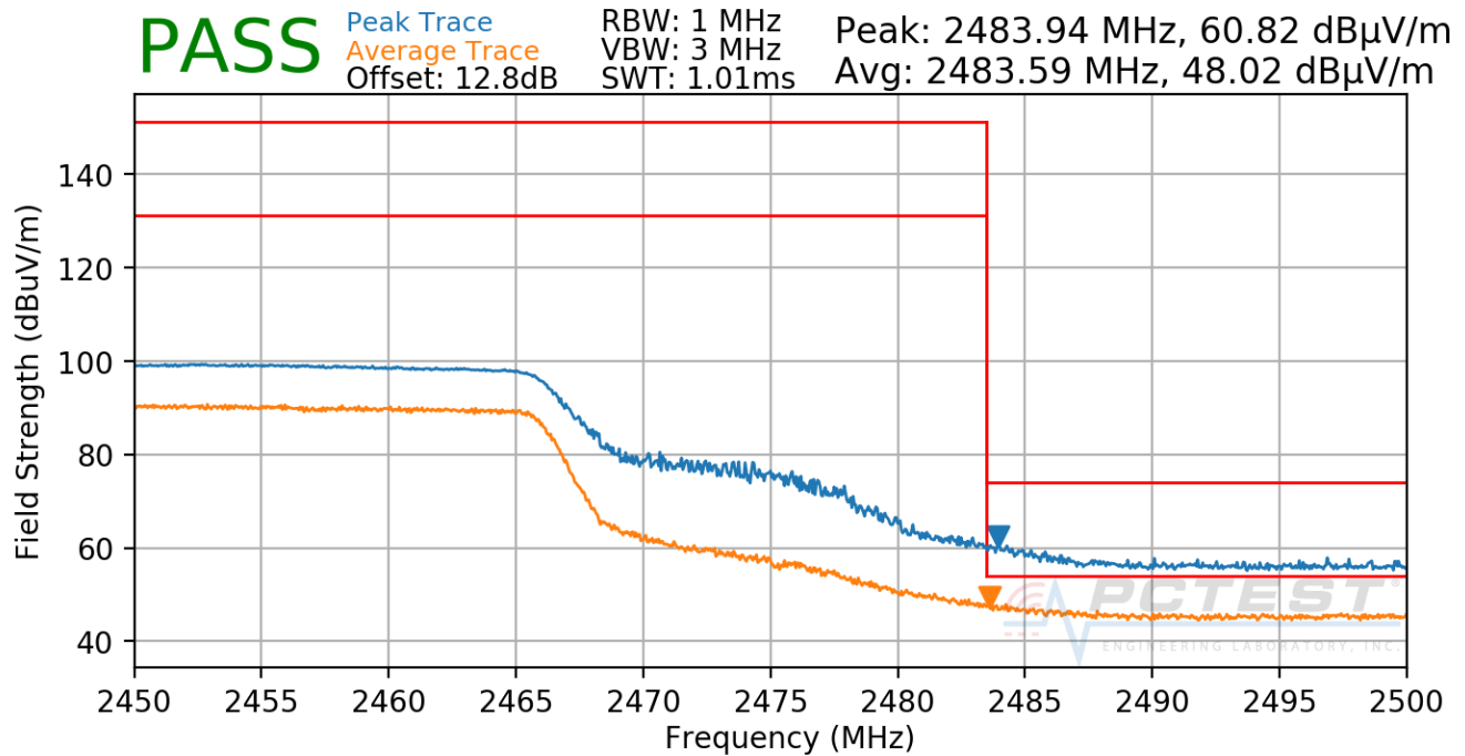
Plot 7-41. Radiated Restricted Upper Band Edge Measurement (Average & Peak)
