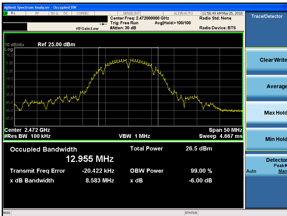
Plot 7-3. 6dB Bandwidth Plot (802.11b – Ch. 13)
