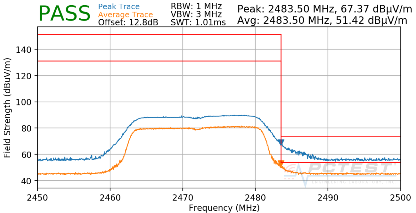
Plot 7-44. Radiated Restricted Upper Band Edge Measurement (Average & Peak)
