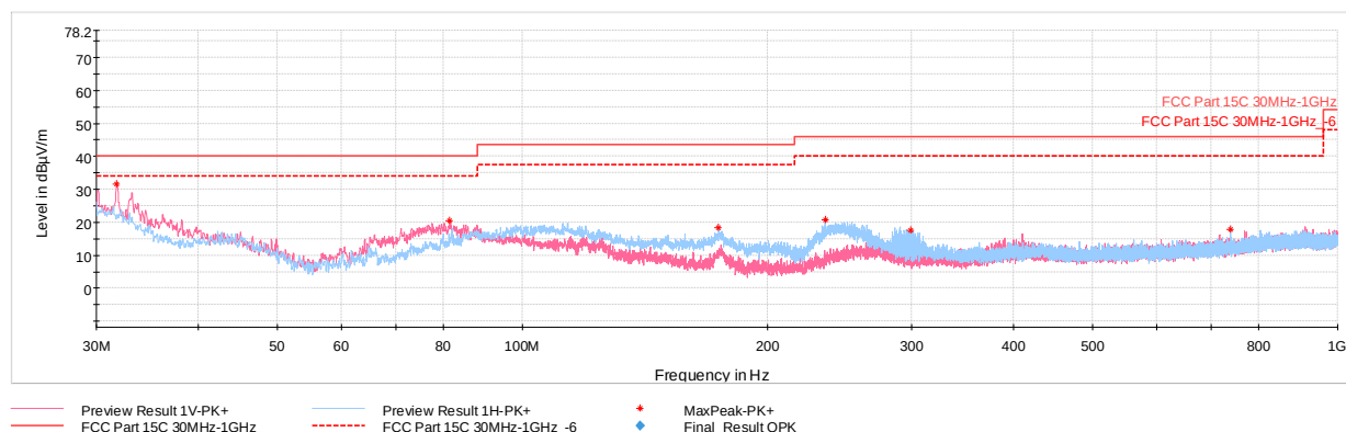
Plot 7-45. Radiated Spurious Plot below 1GHz (802.11b – Ch. 7, Pol. H & V, with WCP + AC/DC Adapter)
