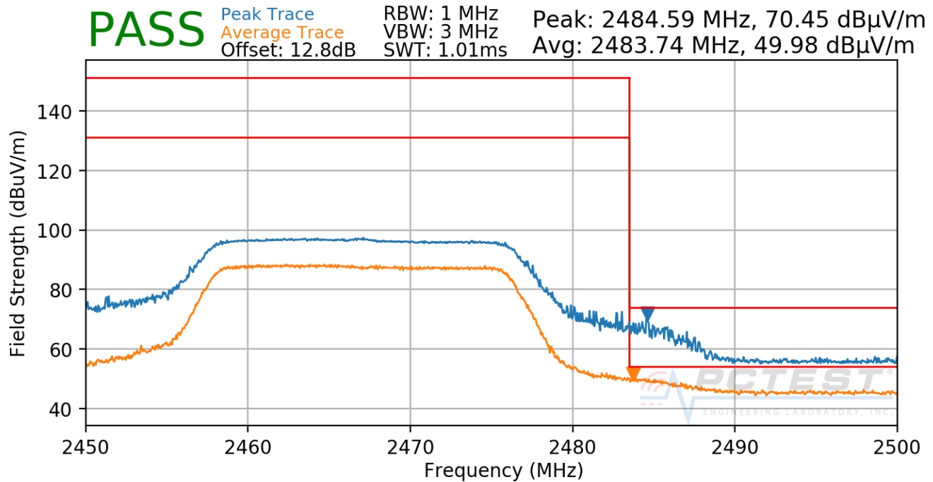
Plot 7-43. Radiated Restricted Upper Band Edge Measurement (Average & Peak)
