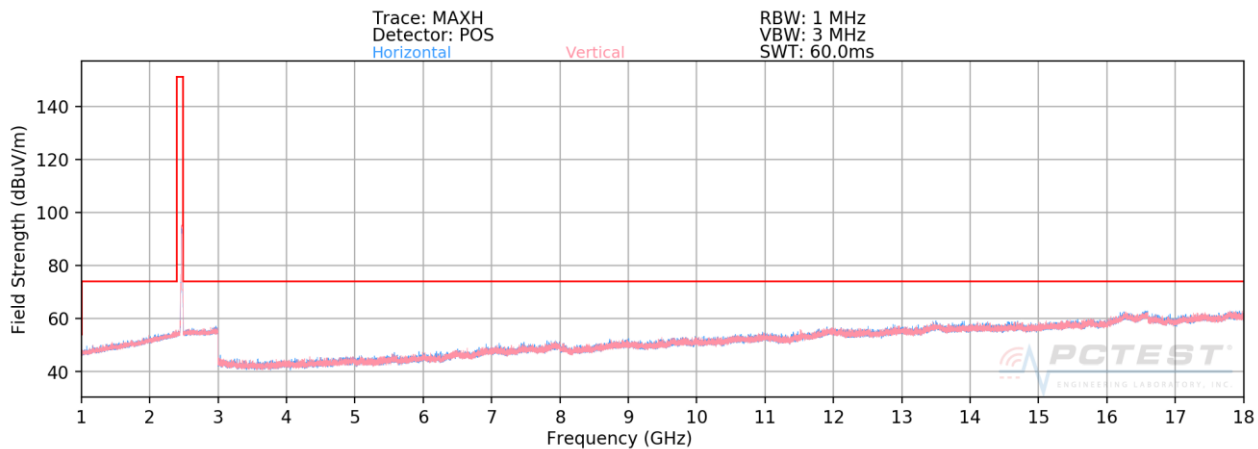
Plot 7-33. Radiated Spurious Plot above 1GHz (802.11b – Ch. 13)
