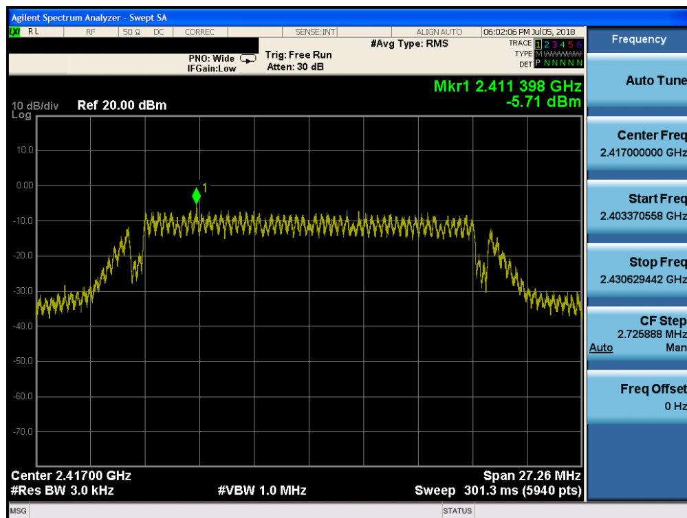
Plot 7-13. Power Spectral Density Plot (802.11g – Ch. 2)
