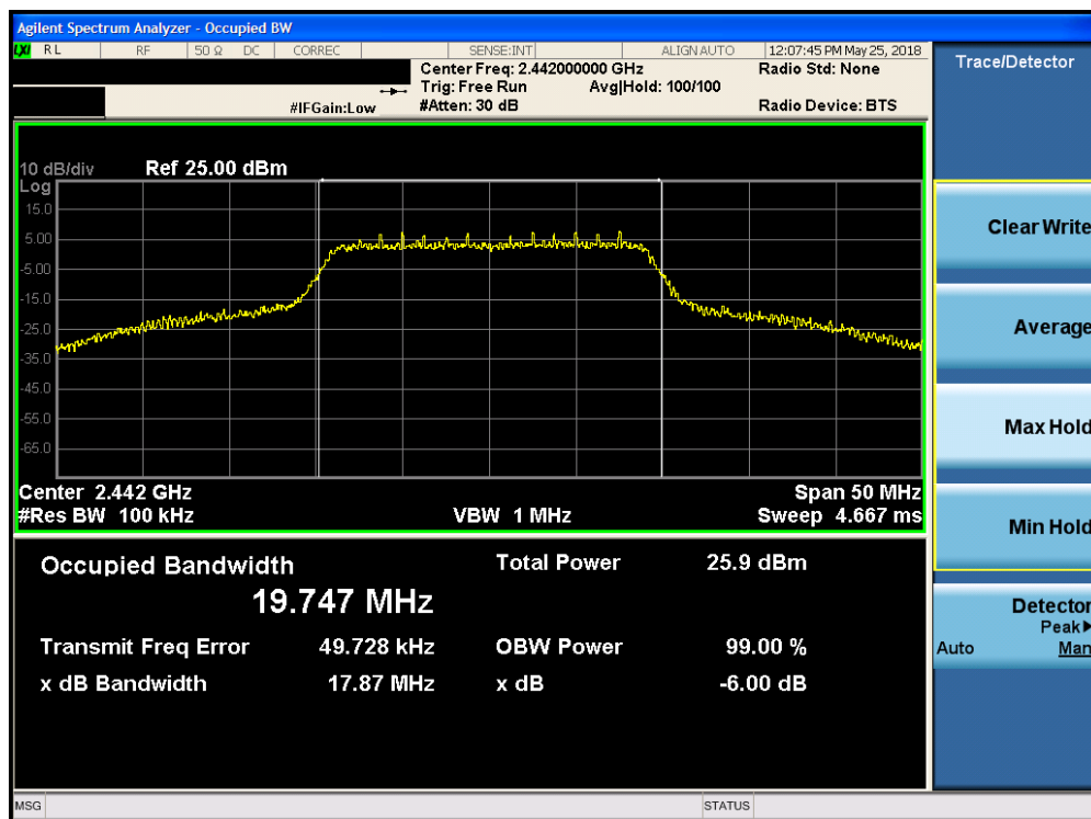
Plot 7-8. 6dB Bandwidth Plot (802.11n (2.4GHz) – Ch. 7)
