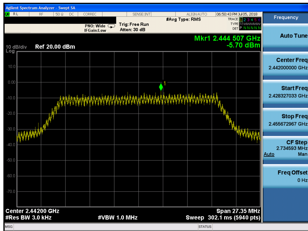
Plot 7-17. Power Spectral Density Plot (802.11n (2.4GHz) – Ch. 7)
