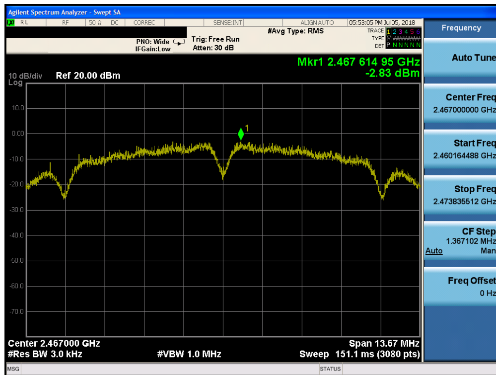
Plot 7-12. Power Spectral Density Plot (802.11b – Ch. 12)
