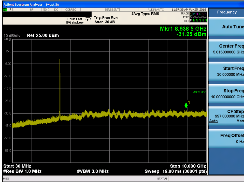
Plot 7-29. Conducted Spurious Plot (802.11b – Ch. 13)
