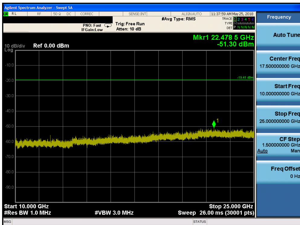
Plot 7-28. Conducted Spurious Plot (802.11b – Ch. 7)
