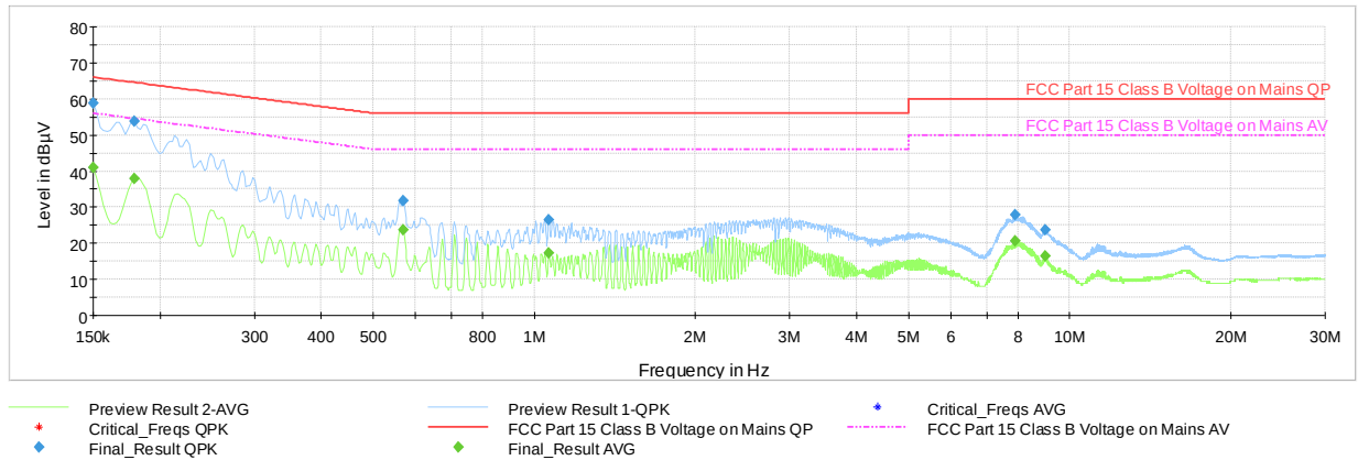
Plot 7-47. Line Conducted Plot with 802.11b (N with WCP + Laptop)
