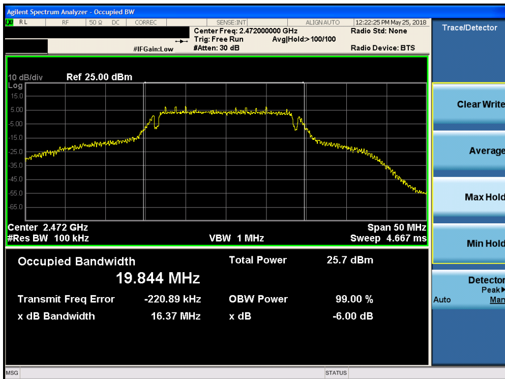
Plot 7-6. 6dB Bandwidth Plot (802.11g – Ch. 13)
