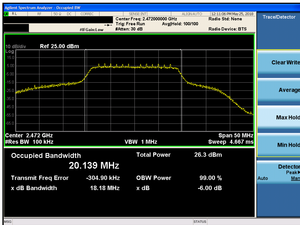
Plot 7-9. 6dB Bandwidth Plot (802.11n (2.4GHz) – Ch. 13)
