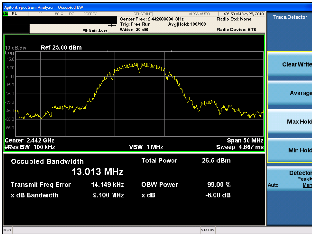
Plot 7-2. 6dB Bandwidth Plot (802.11b – Ch. 7)
