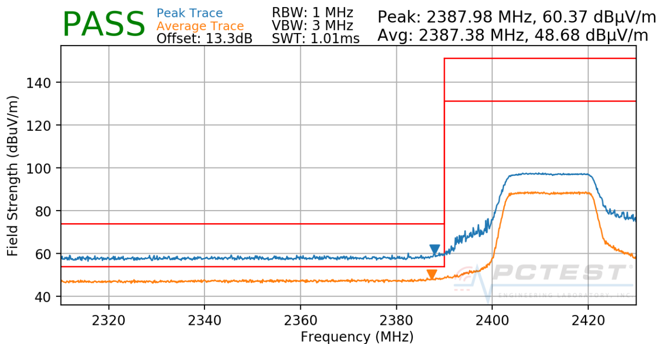
Plot 7-39. Radiated Restricted Lower Band Edge Measurement (Average & Peak)
