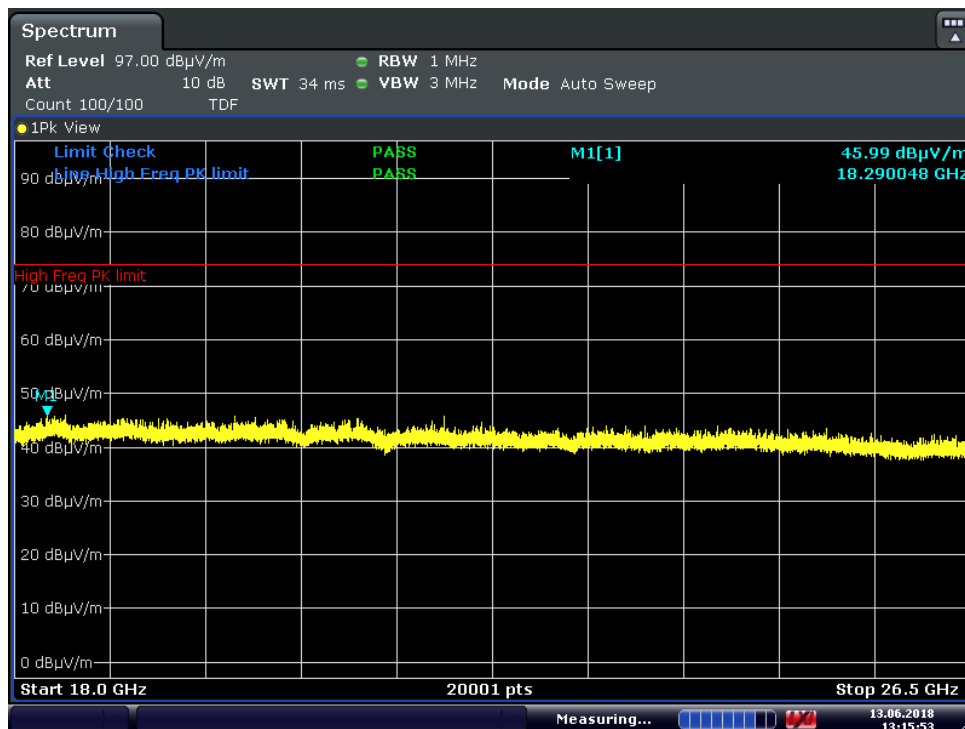
Plot 7-35. Radiated Spurious Plot above 18GHz (802.11b – Ch. 7, Ant. Pol. V)
