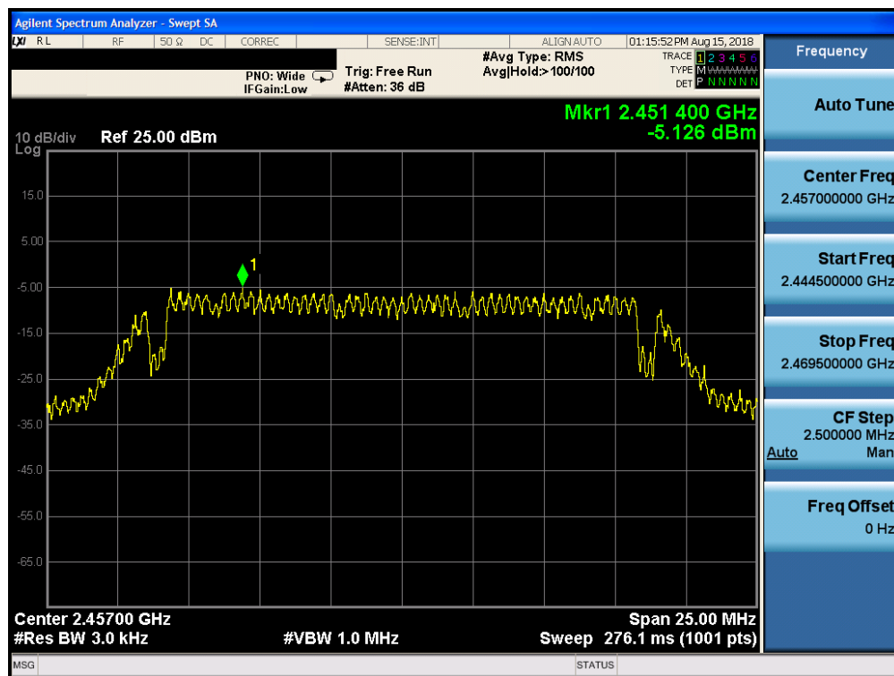
Plot 7-15. Power Spectral Density Plot (802.11g – Ch. 10)
