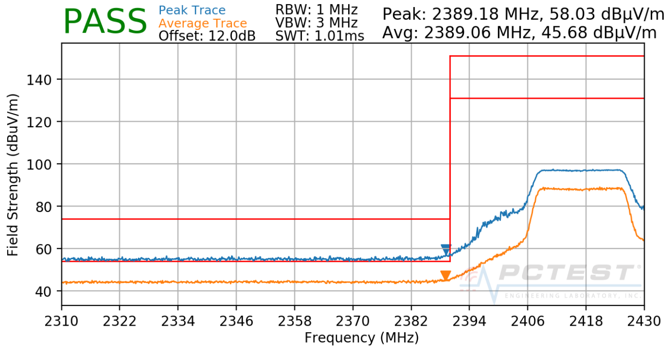
Plot 7-40. Radiated Restricted Lower Band Edge Measurement (Average & Peak)
