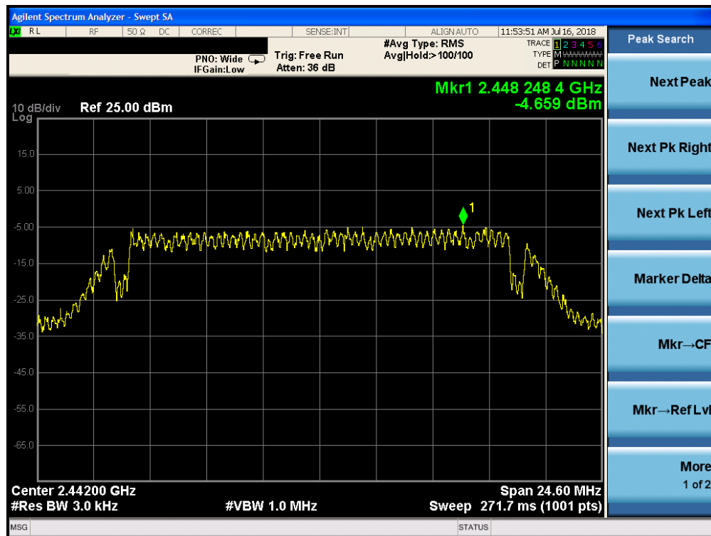
Plot 7-14. Power Spectral Density Plot (802.11g – Ch. 7)
