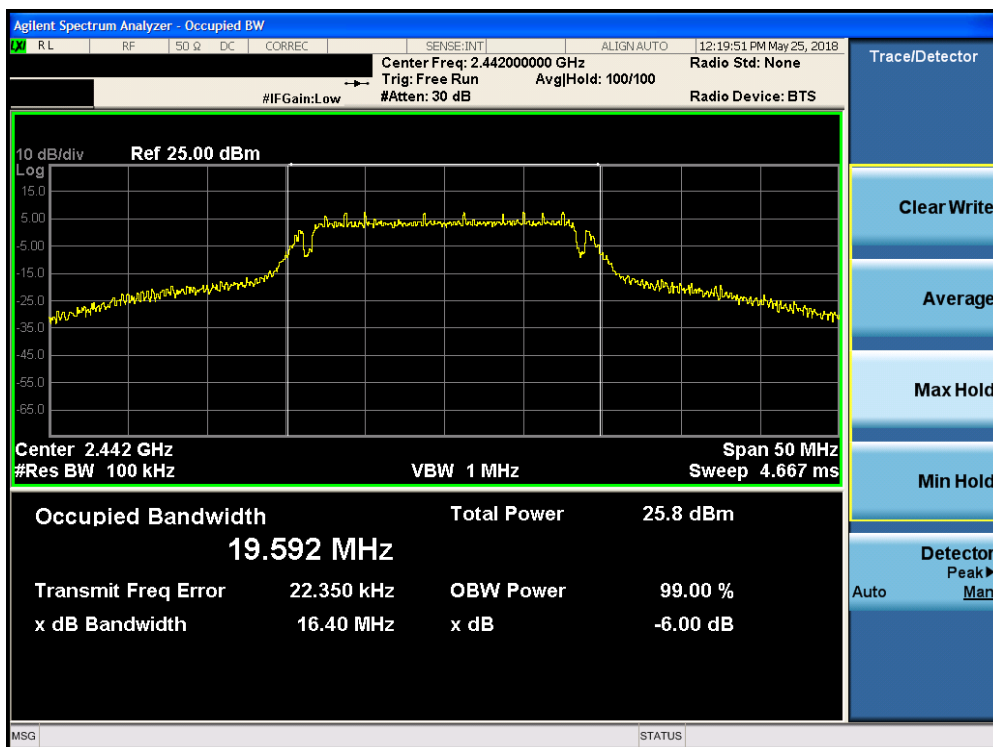
Plot 7-5. 6dB Bandwidth Plot (802.11g – Ch. 7)
