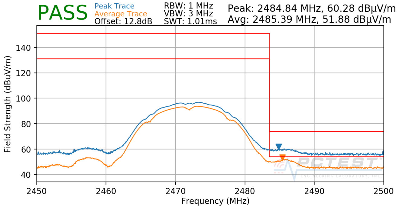
Plot 7-38. Radiated Restricted Upper Band Edge Measurement (Average & Peak)
