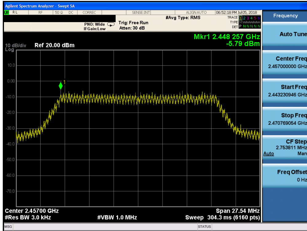
Plot 7-18. Power Spectral Density Plot (802.11n (2.4GHz) – Ch. 10)
