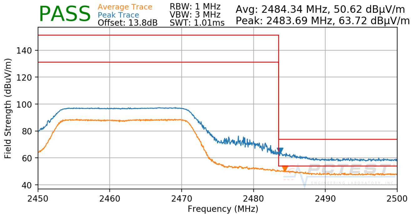
Plot 7-42. Radiated Restricted Upper Band Edge Measurement (Average & Peak)
