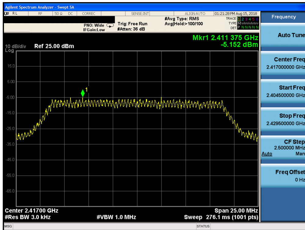
Plot 7-16. Power Spectral Density Plot (802.11n (2.4GHz) – Ch. 2)
