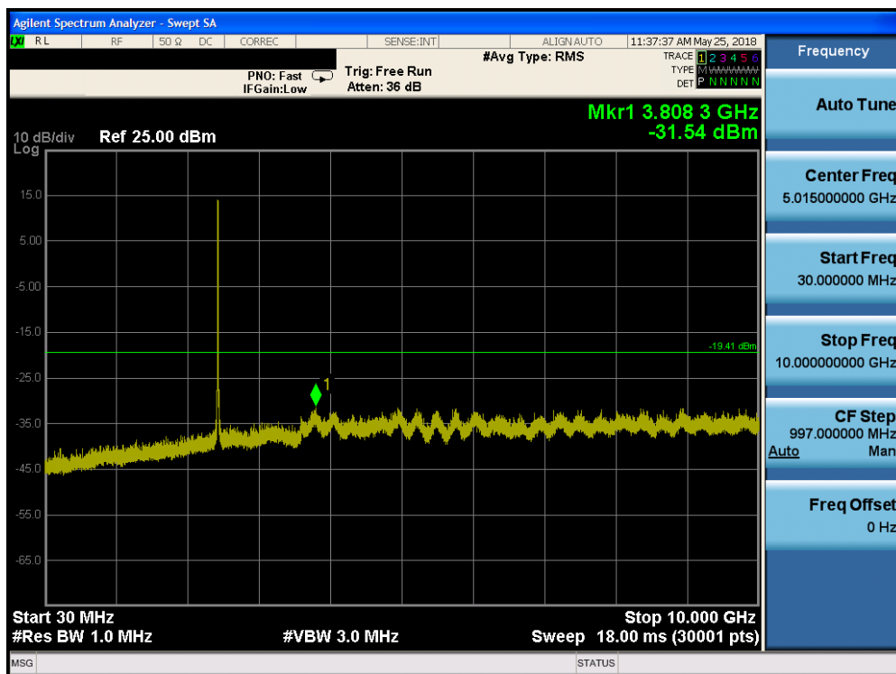
Plot 7-27. Conducted Spurious Plot (802.11b – Ch. 7)
