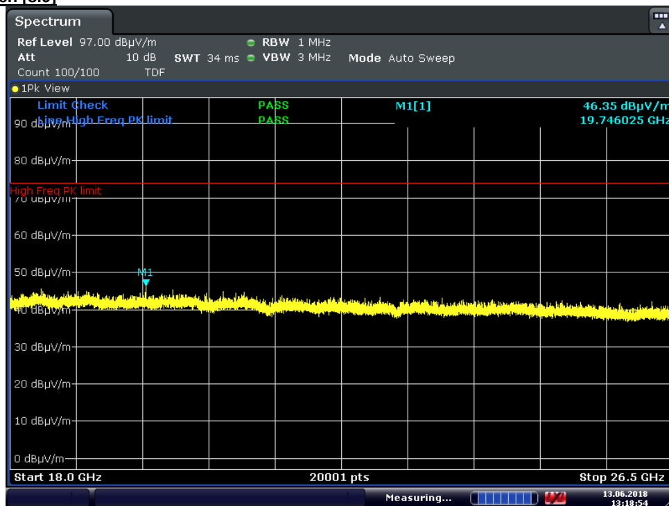
Plot 7-34. Radiated Spurious Plot above 18GHz (802.11b – Ch. 7, Ant. Pol. H)
