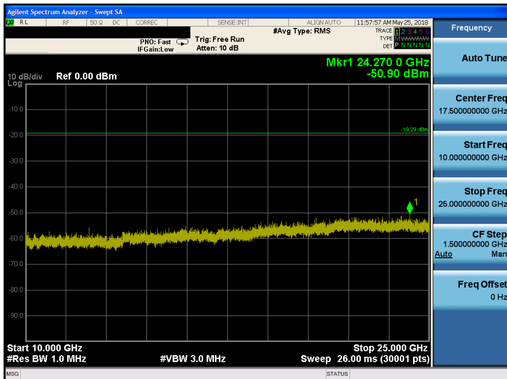
Plot 7-30. Conducted Spurious Plot (802.11b – Ch. 13)
