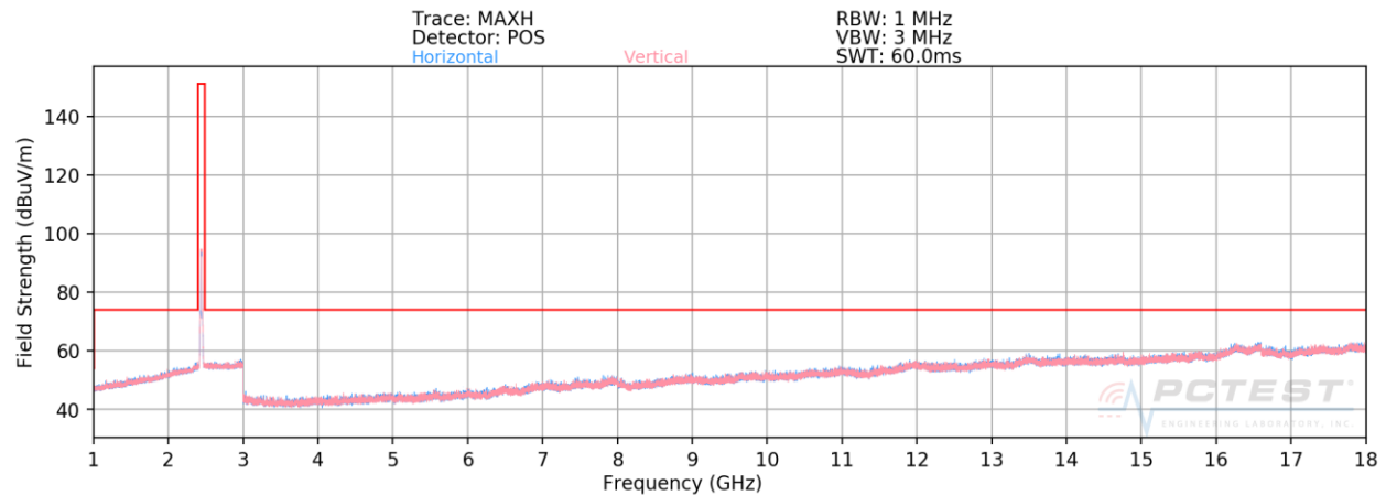
Plot 7-32. Radiated Spurious Plot above 1GHz (802.11b – Ch. 7)
