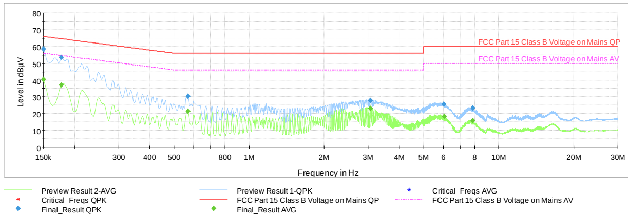
Plot 7-46. Line Conducted Plot with 802.11b (L1, with WCP + Laptop)
