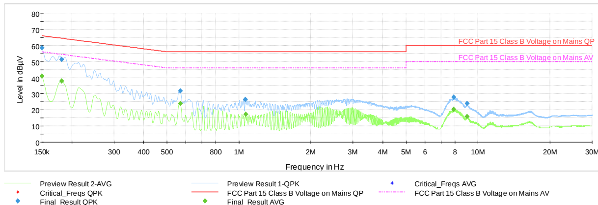
Plot 7-56. Line Conducted Plot with Bluetooth LE (N, with WCP + Laptop)
