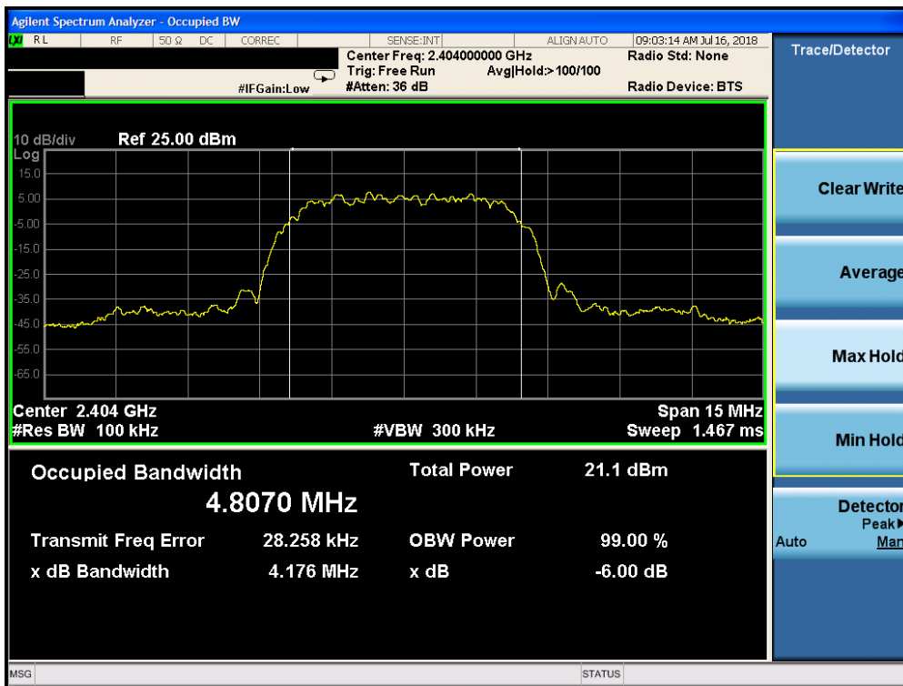
Plot 7-10. 6dB Bandwidth Plot (Bluetooth (HDR, ePA), 8Mbps – Ch. 1)
