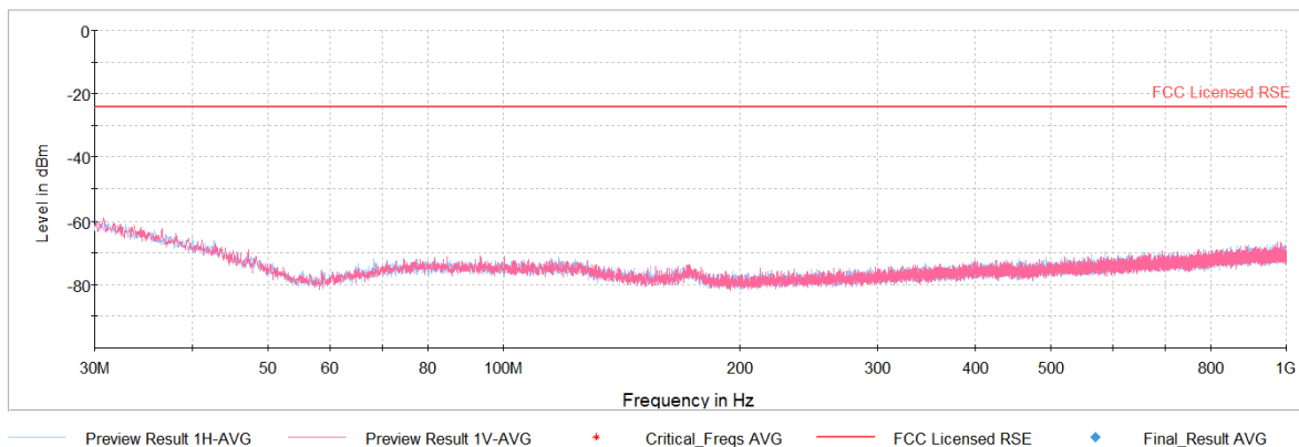
Plot 7-26. Radiated Spurious Plot (Band 41 – 15.0MHz QPSK – RB Size 75)
