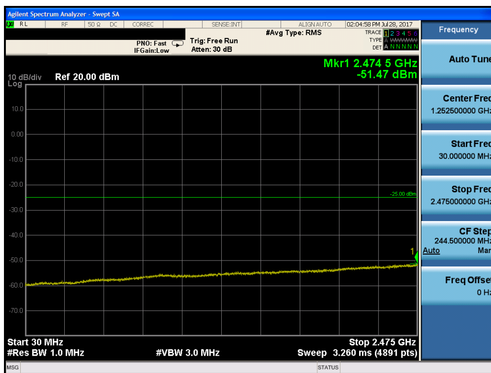
Plot 7-26. Conducted Spurious Plot (Band 7 – 5.0MHz QPSK – RB Size 1, RB Offset 0 – Low Channel)
