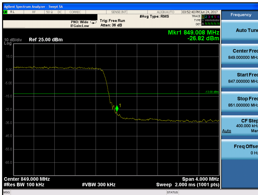
Plot 7-40. Upper Band Edge Plot (Band 5/26 – 5.0MHz QPSK – RB Size 25)
