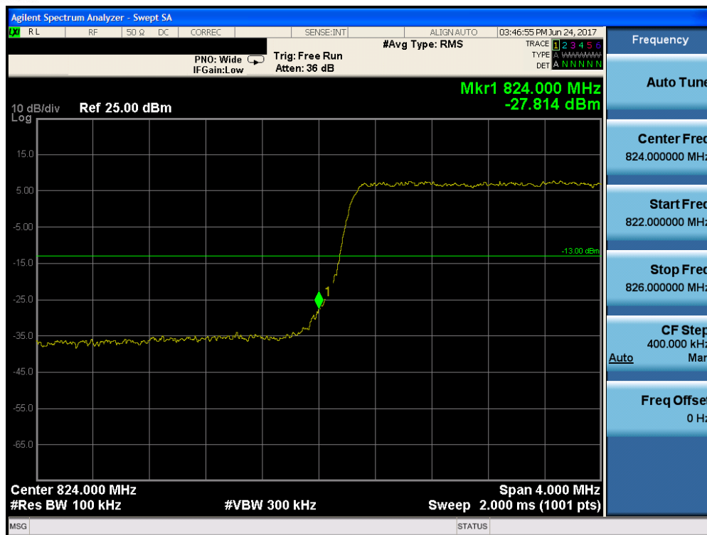
Plot 7-39. Lower Band Edge Plot (Band 5/26 – 5.0MHz QPSK – RB Size 25)
