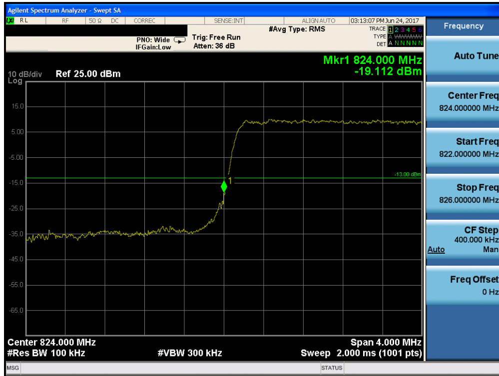
Plot 7-37. Lower Band Edge Plot (Band 5/26 - 3.0MHz QPSK - RB Size 15)
