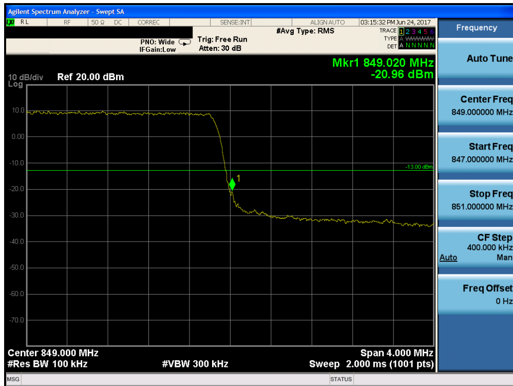
Plot 7-38. Upper Band Edge Plot (Band 5/26 - 3.0MHz QPSK - RB Size 15)
