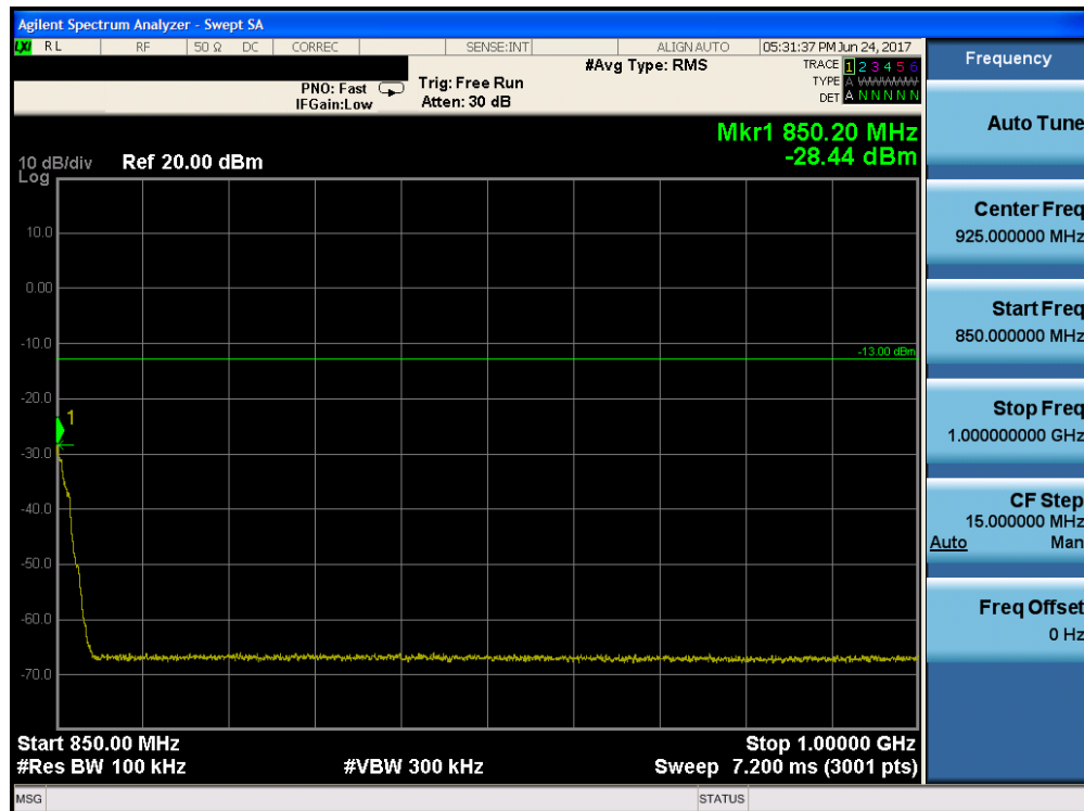
Plot 7-9. Conducted Spurious Plot (Cellular WCDMA Mode – Ch. 4233)
