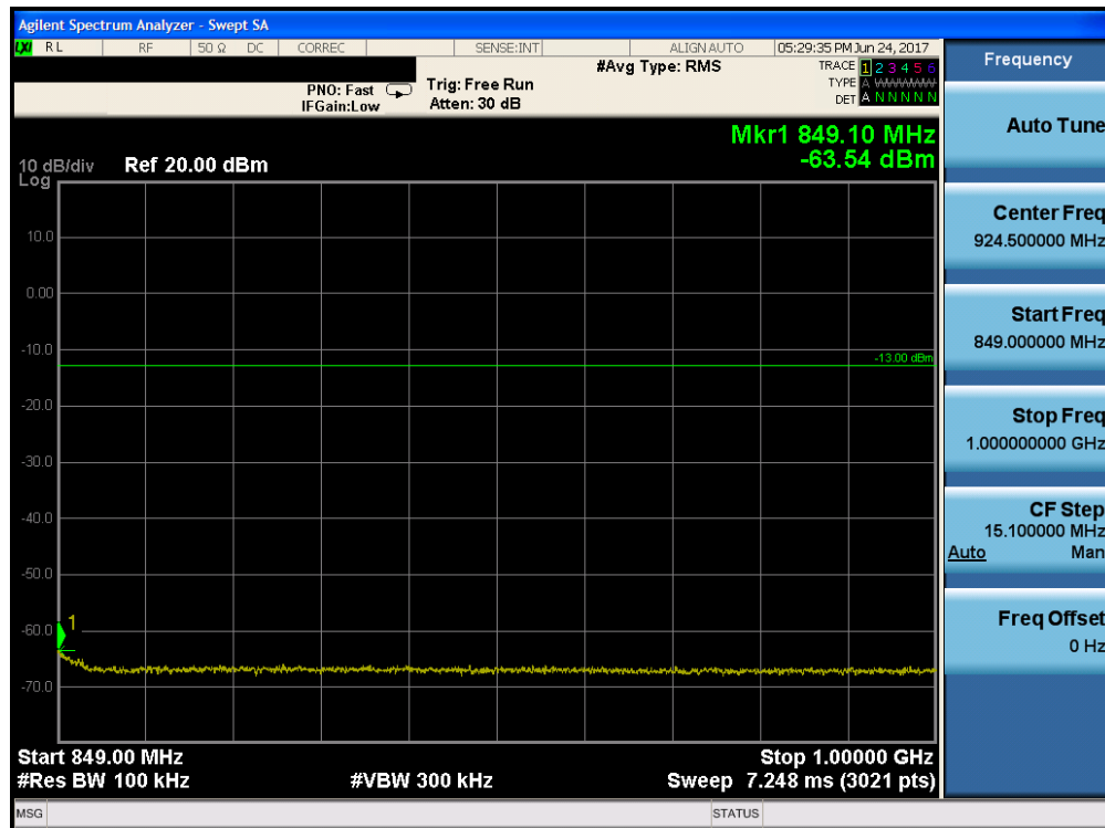
Plot 7-3. Conducted Spurious Plot (Cellular WCDMA Mode – Ch. 4132)
