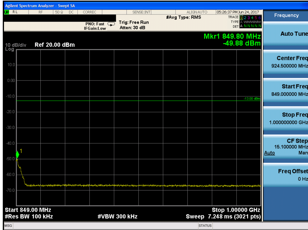
Plot 7-6. Conducted Spurious Plot (Cellular WCDMA Mode – Ch. 4183)
