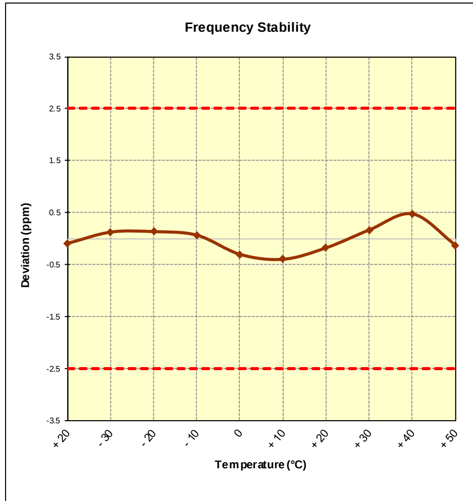
Figure 7-7. Frequency Stability Graph (Cellular WCDMA Mode – Ch. 4183)
