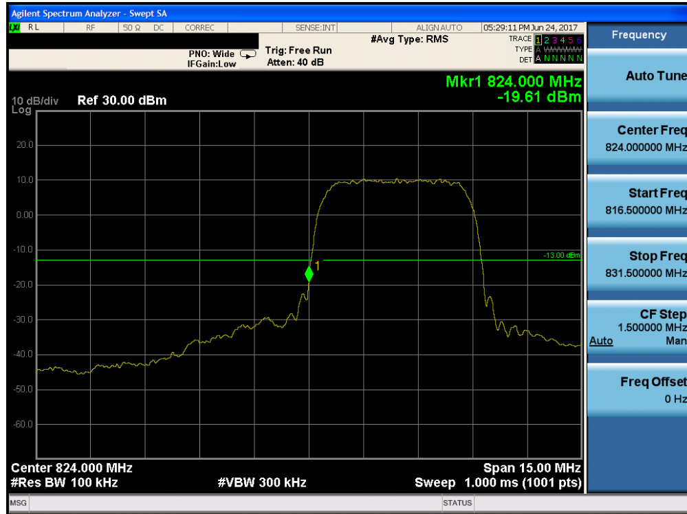
Plot 7-11. Band Edge Plot (Cellular WCDMA Mode – Ch. 4132)
