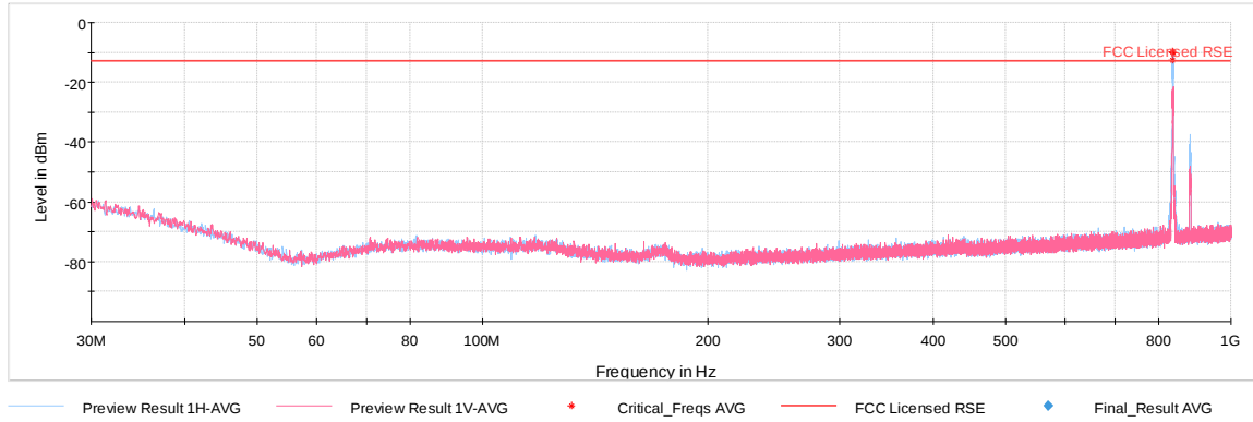
Plot 7-13. Radiated Spurious Plot (Cellular WCDMA Mode – Ch. 4183)
