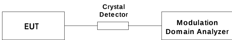
Test Set-up 2
