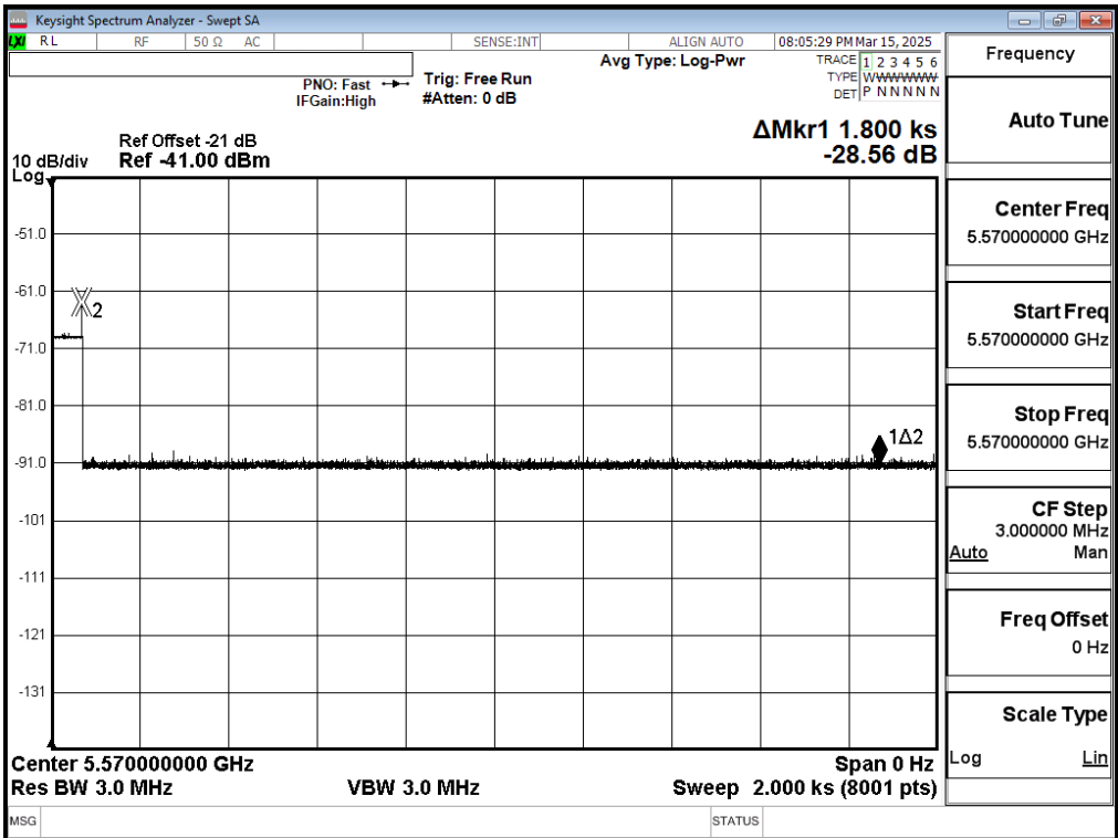
Non-Occupancy Period - 802.11ax (160 MHz), 5570 MHz
