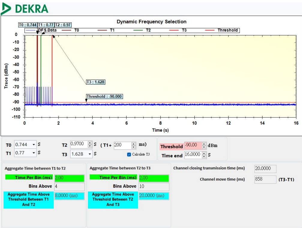
Channel Move Time and Channel Closing Transmission Time - 802.11ax (160 MHz), 5570 MHz
