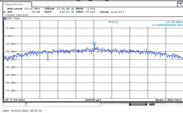
BLE_2M_Ant1_2440
