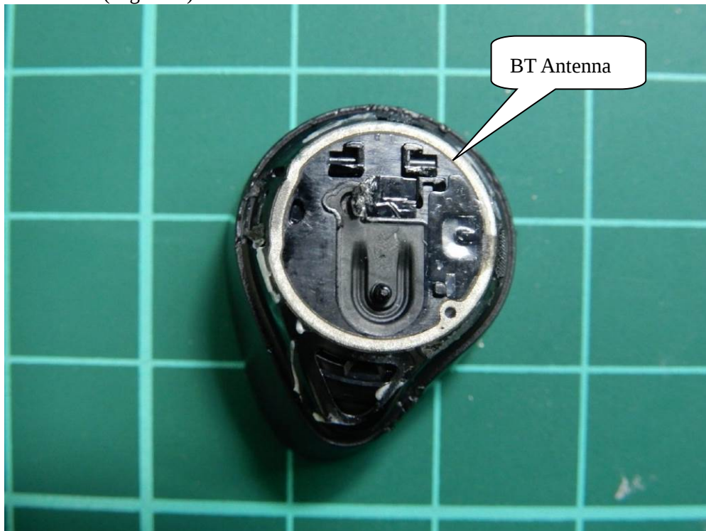
(4) EUT Photo (Right ear)
