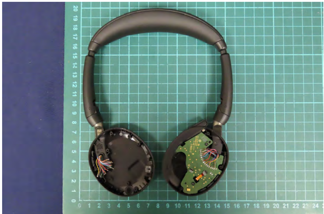
(28) EUT Photo
