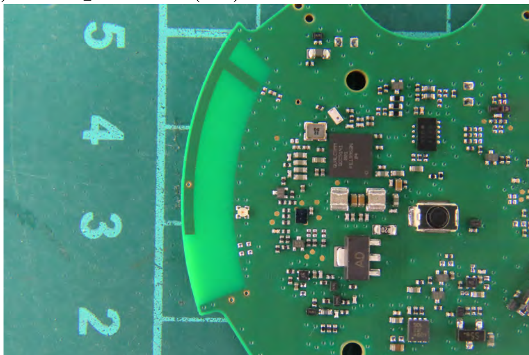
(52) EUT Photo _M/N: HSC170W (mono)
