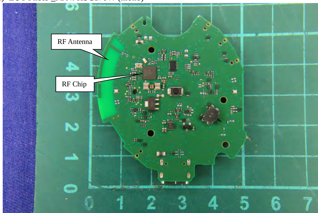
(51) EUT Photo _M/N: HSC170W (mono)
