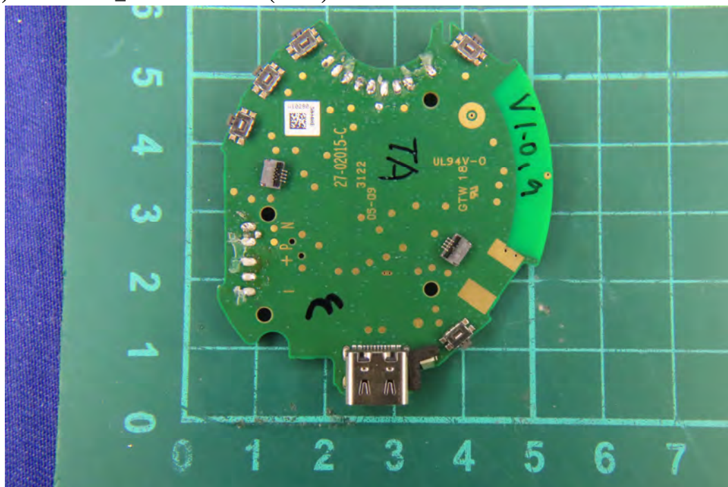
(50) EUT Photo _M/N: HSC170W (mono)
