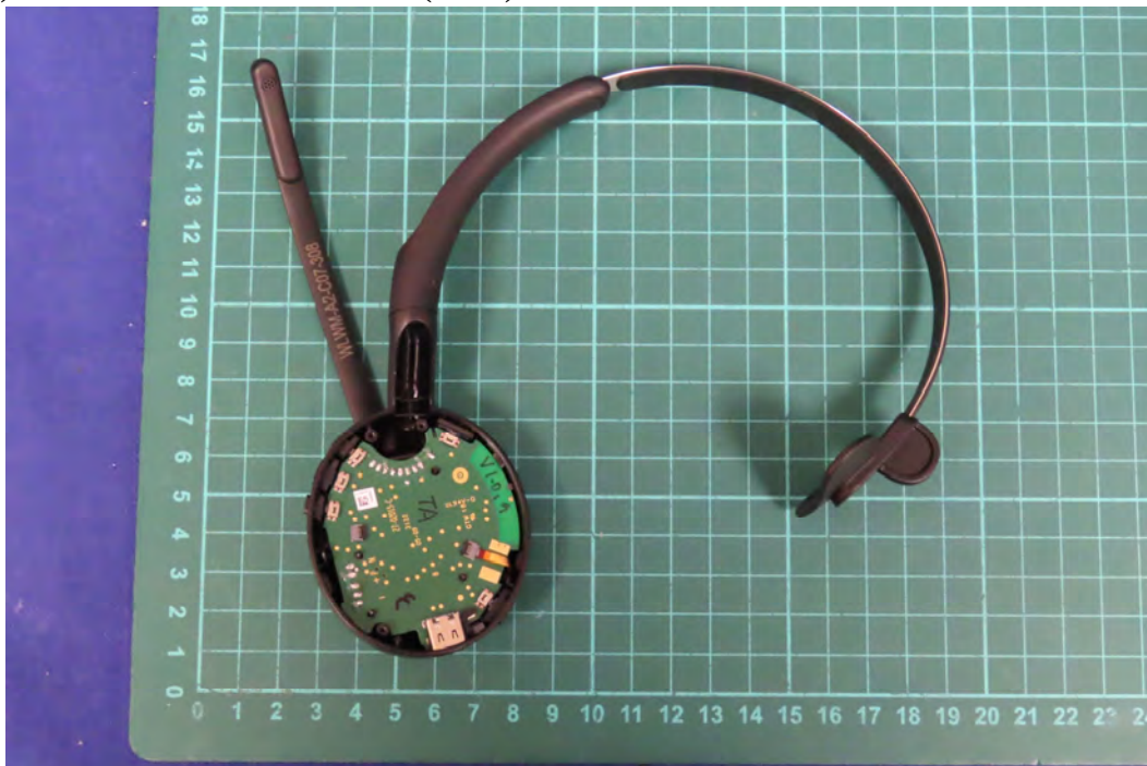
(48) EUT Photo _M/N: HSC170W (mono)
