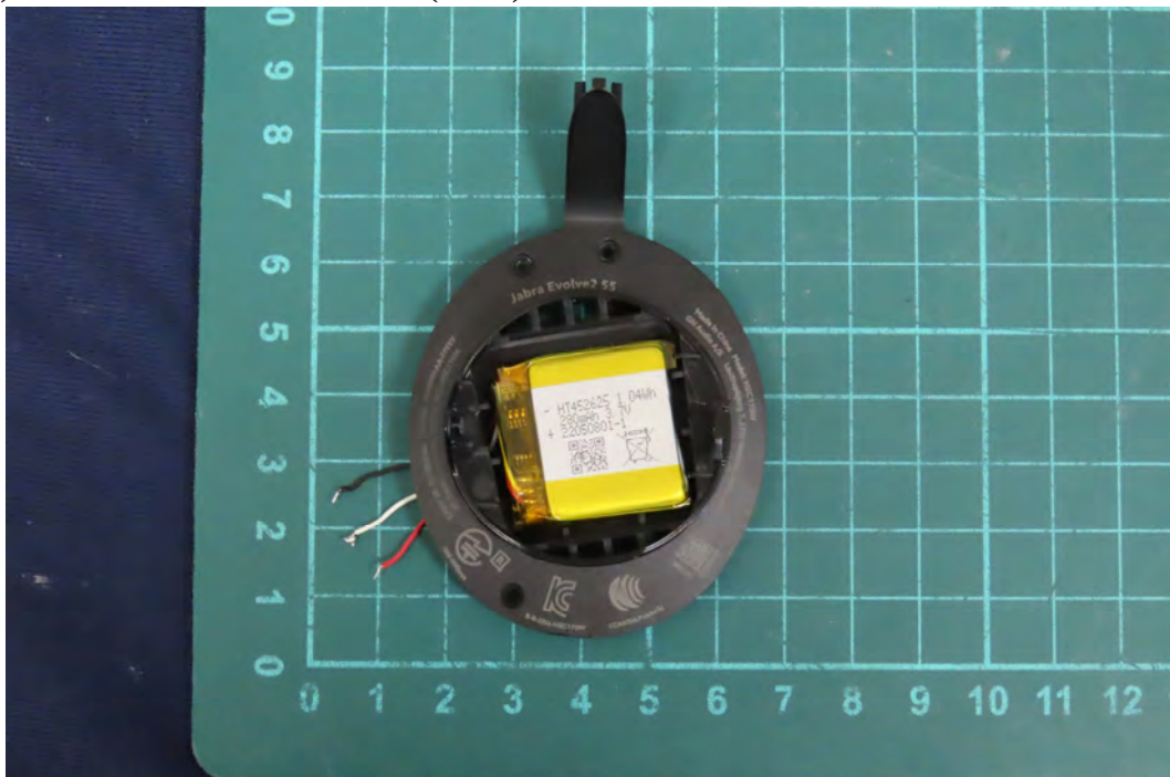
(42) EUT Photo _M/N: HSC170W (mono)
