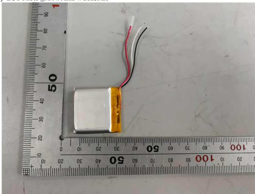
(17) EUT Photo _M/N: AHB472625PLT
