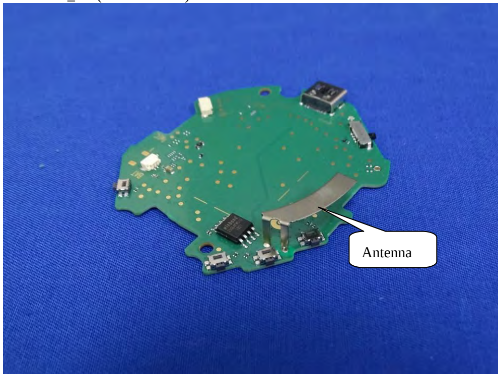
(82) EUT Photo _ant (stereo headset)
