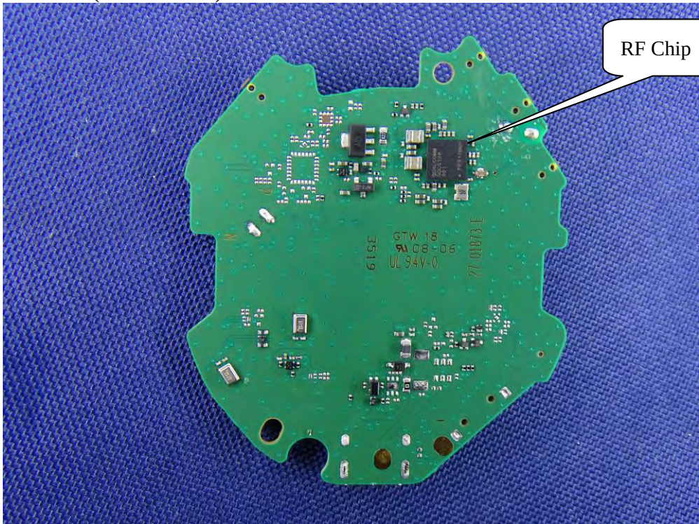
(84) EUT Photo (stereo headset)
