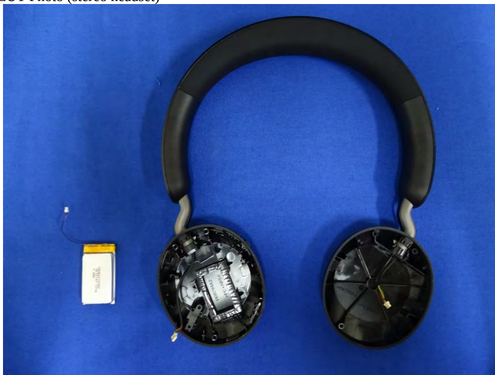
(87) EUT Photo (stereo headset)
