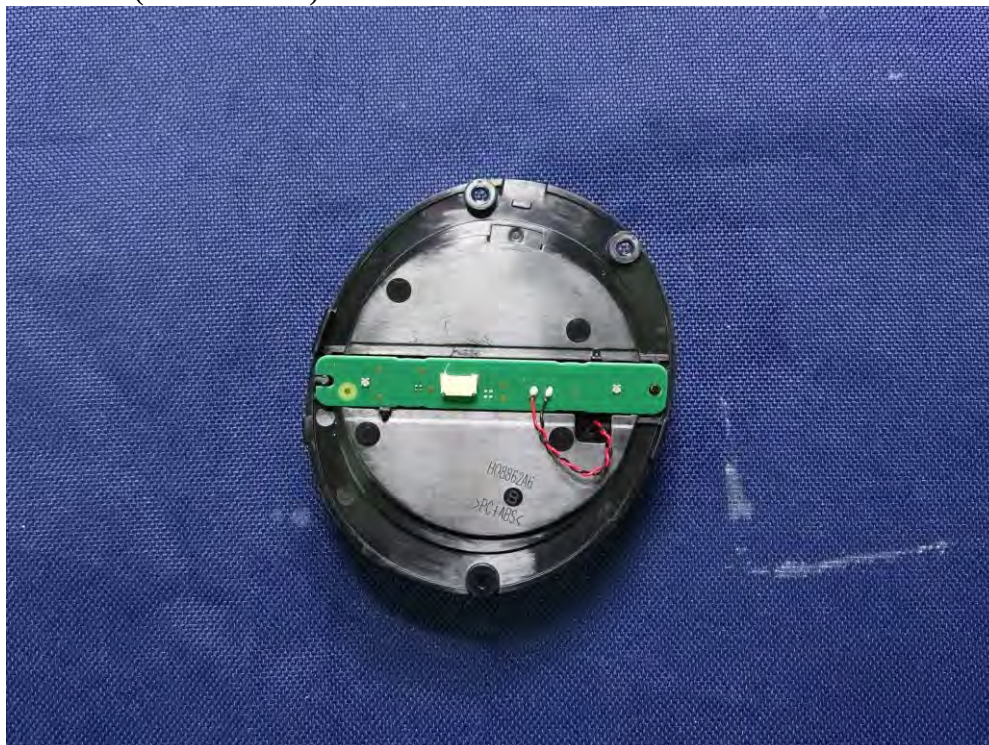
(76) EUT Photo (stereo headset)
