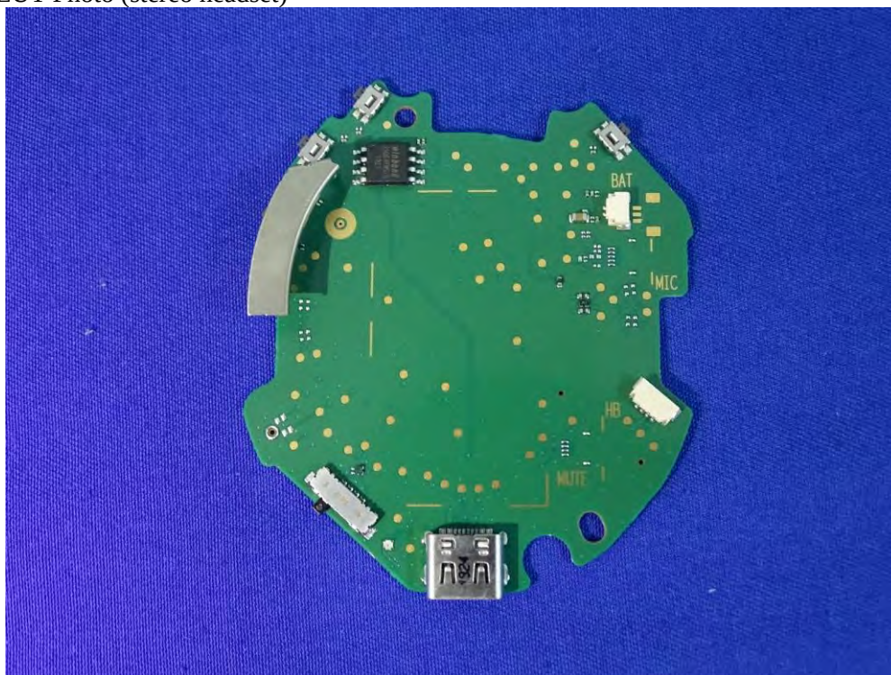
(81) EUT Photo (stereo headset)
