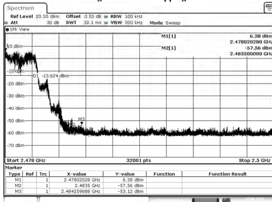
Figure Channel Hopping:
