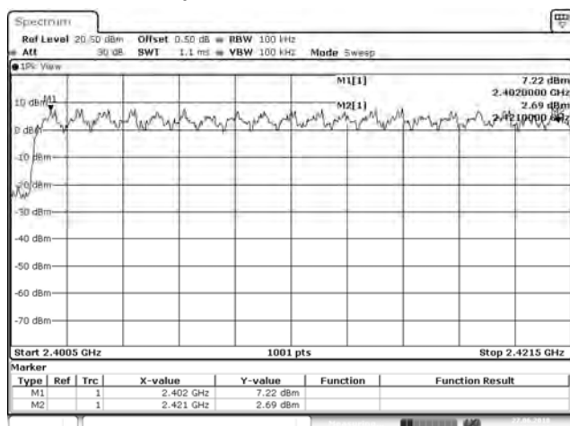
2402-2421MHz
