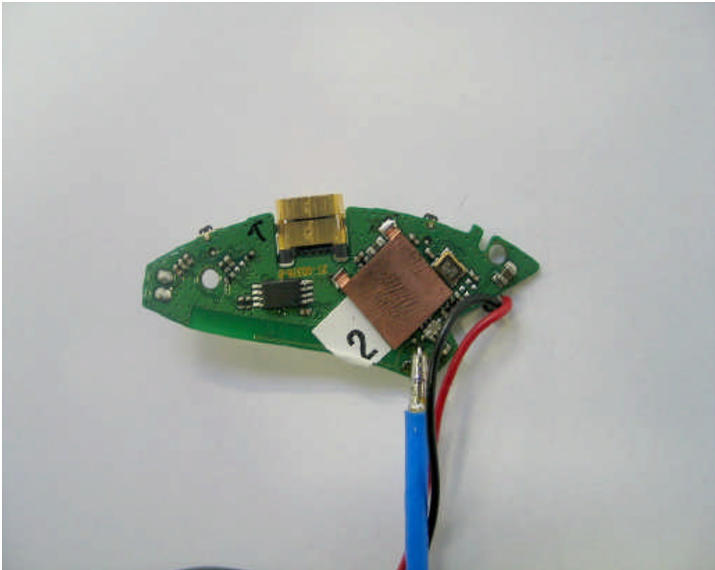
Photo 7: PCB of EUT (top side, with temporary antenna connector)
