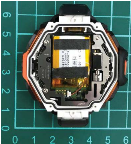
Module in Watch case (with Battery)
