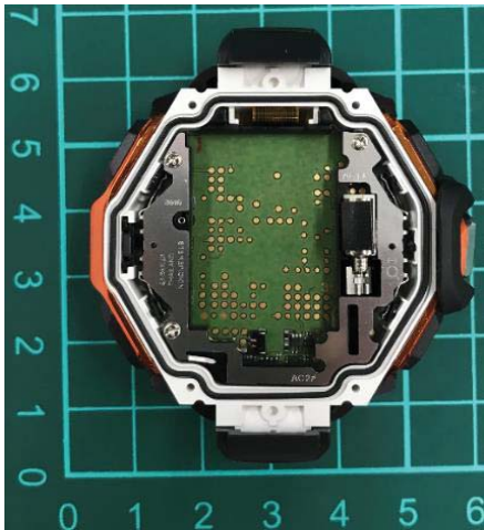
Module in Watch case (with Metal Plate)
