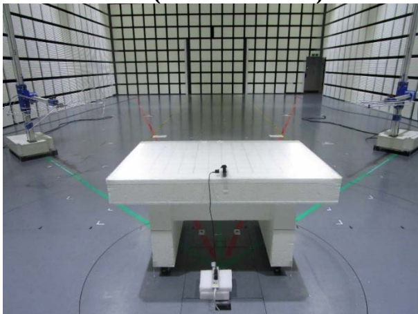
Rear (30 MHz - 1 GHz)
