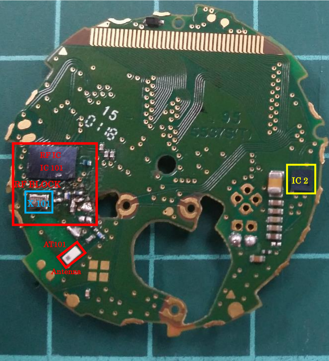
Front side
