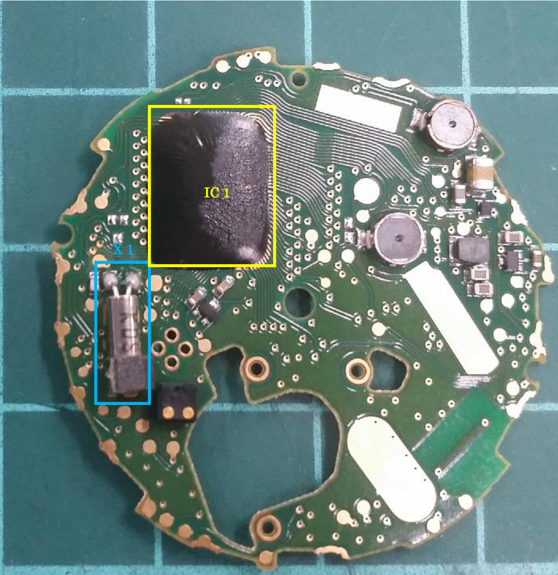
Back side
