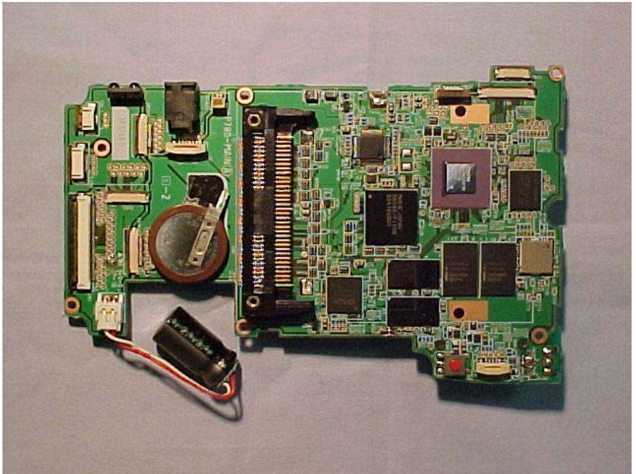
Main Board Underside without Shielding
