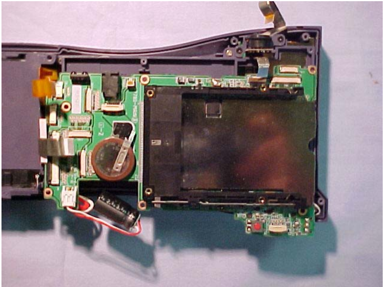
Main Board Underside with Shielding
