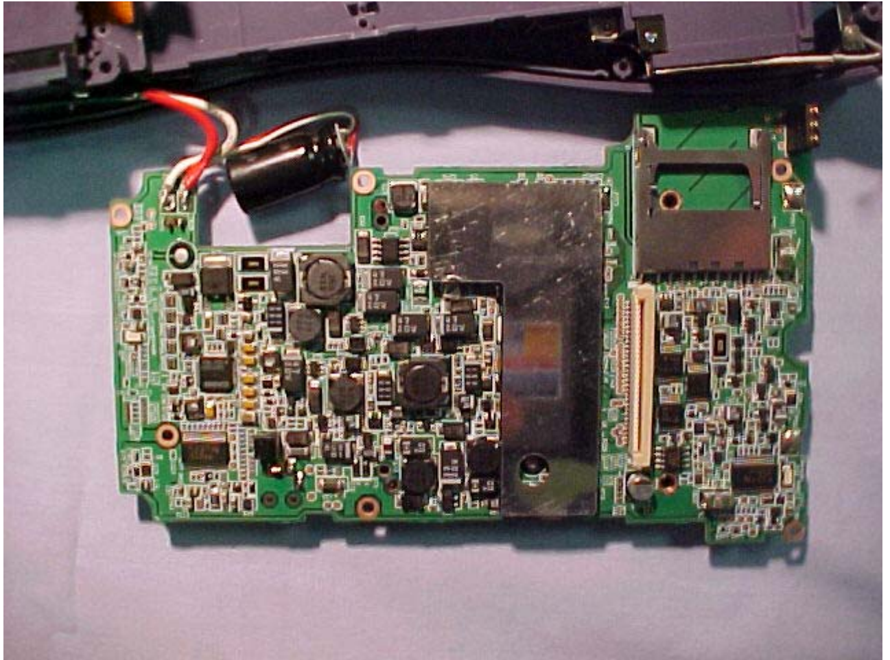
Main Board Top with Shielding
