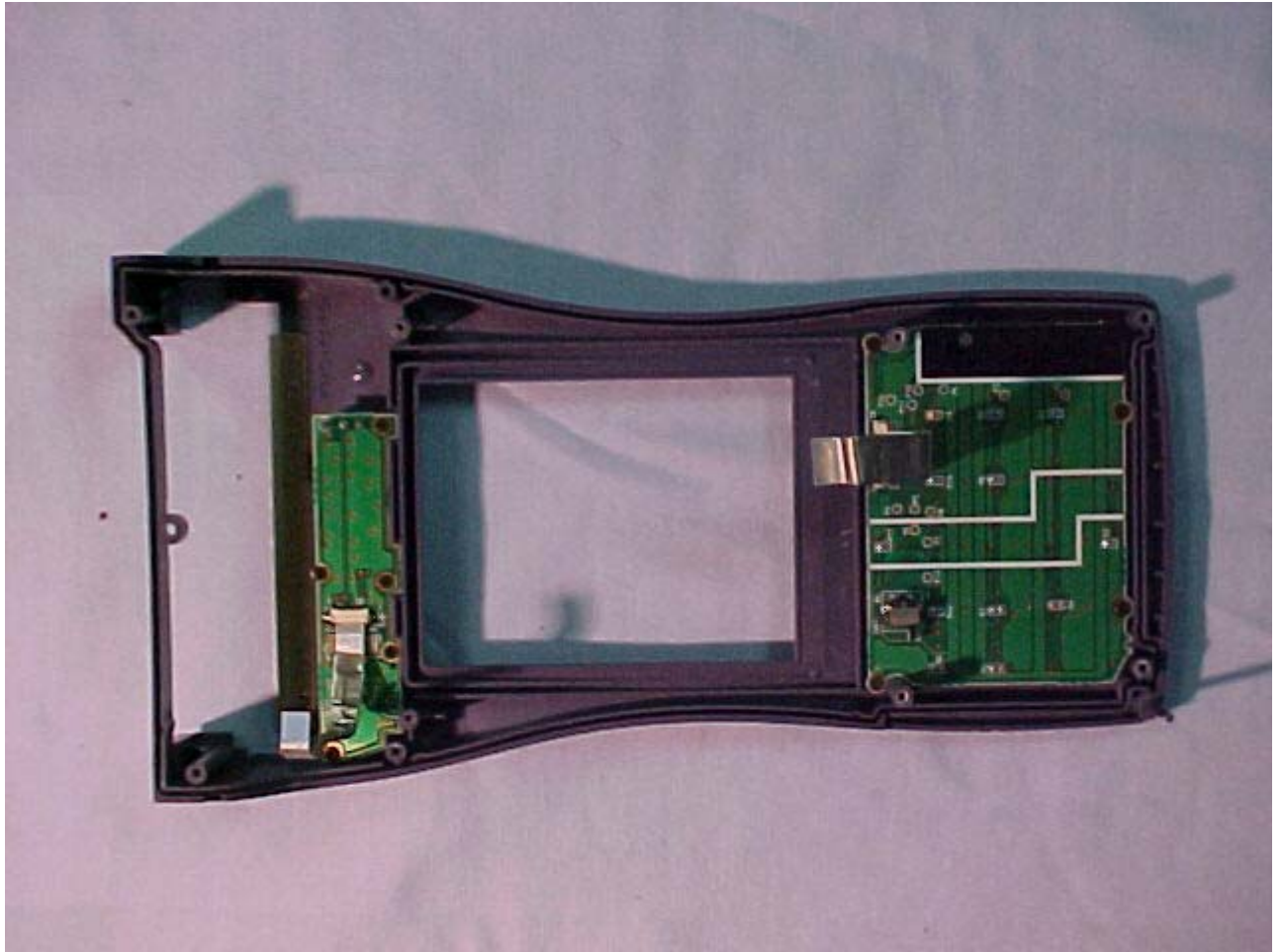
Keyboard and on/off switch assembly
