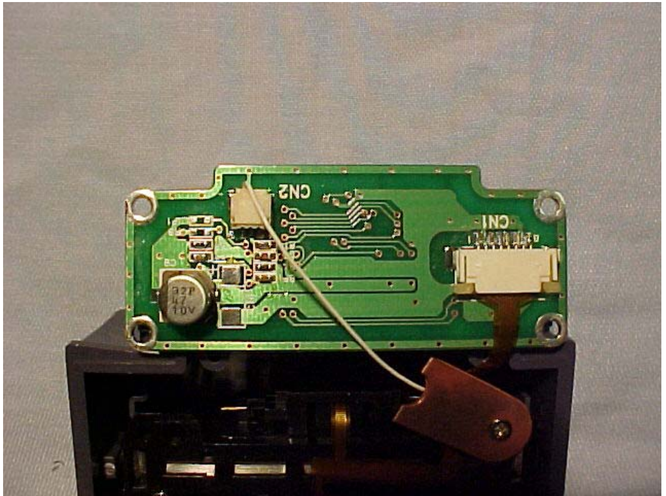
Magnetic Card Reader Interface Top
