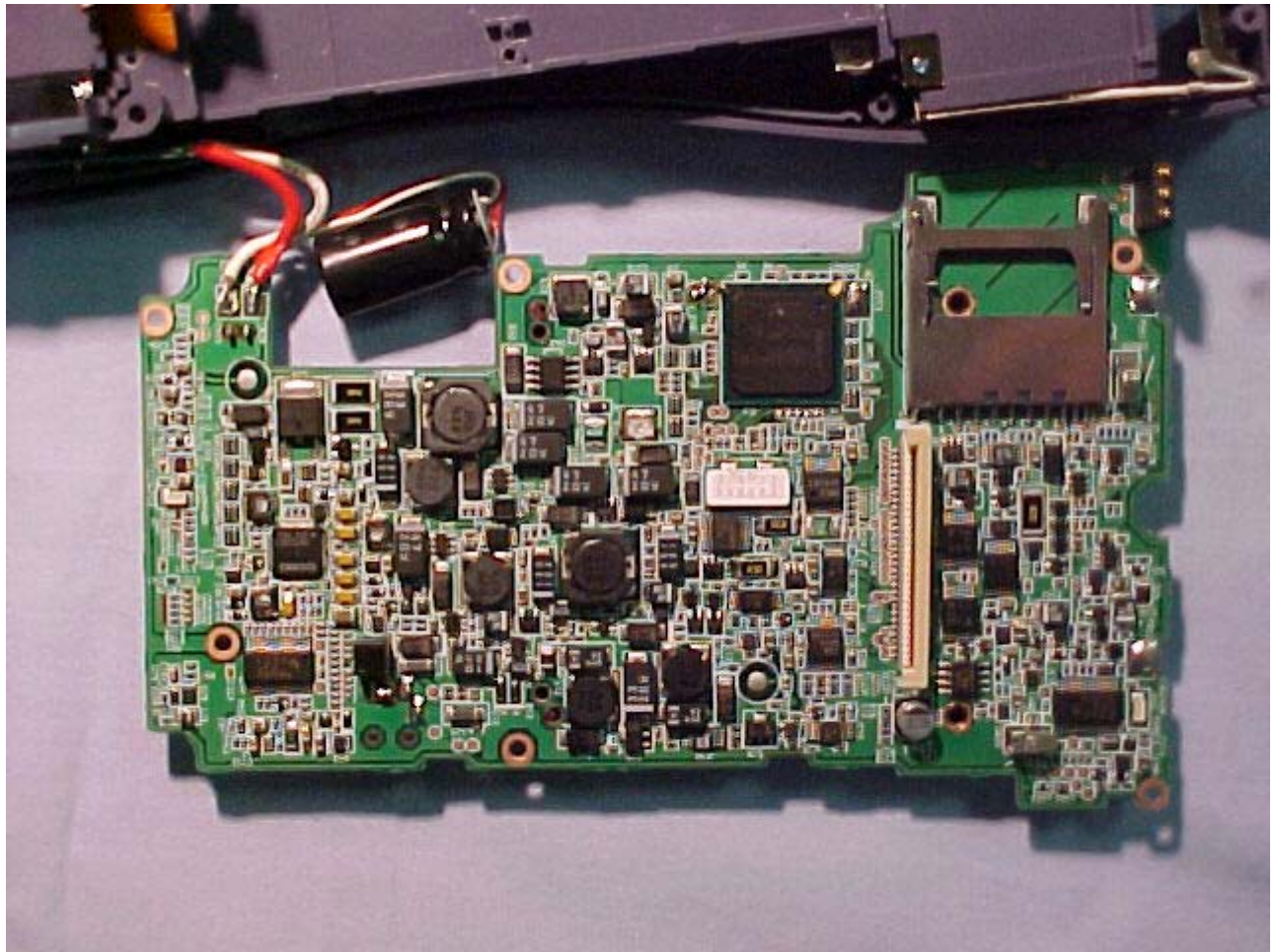
Main Board Top without Shielding
