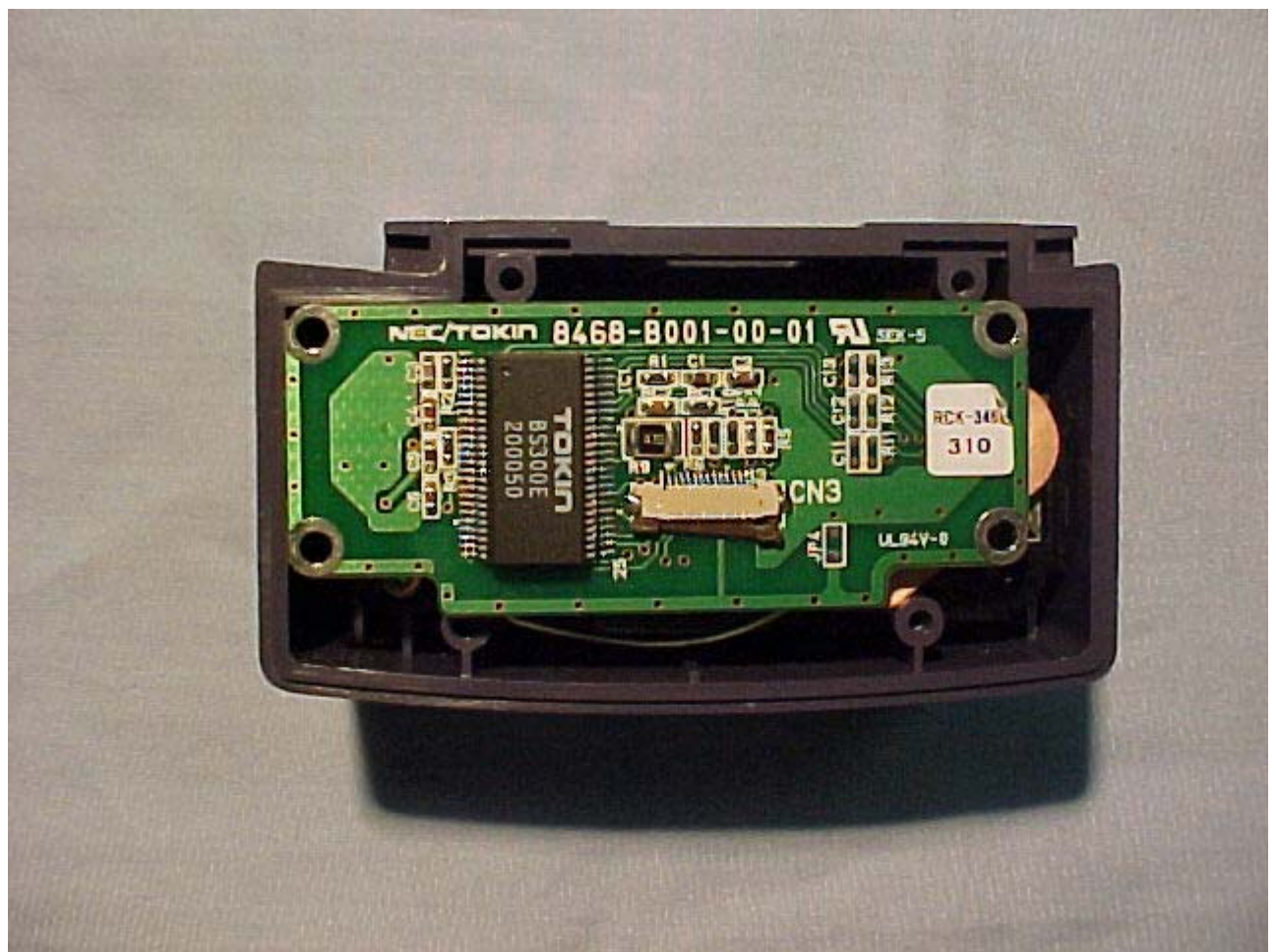
Magnetic Card Reader Interface Bottom
