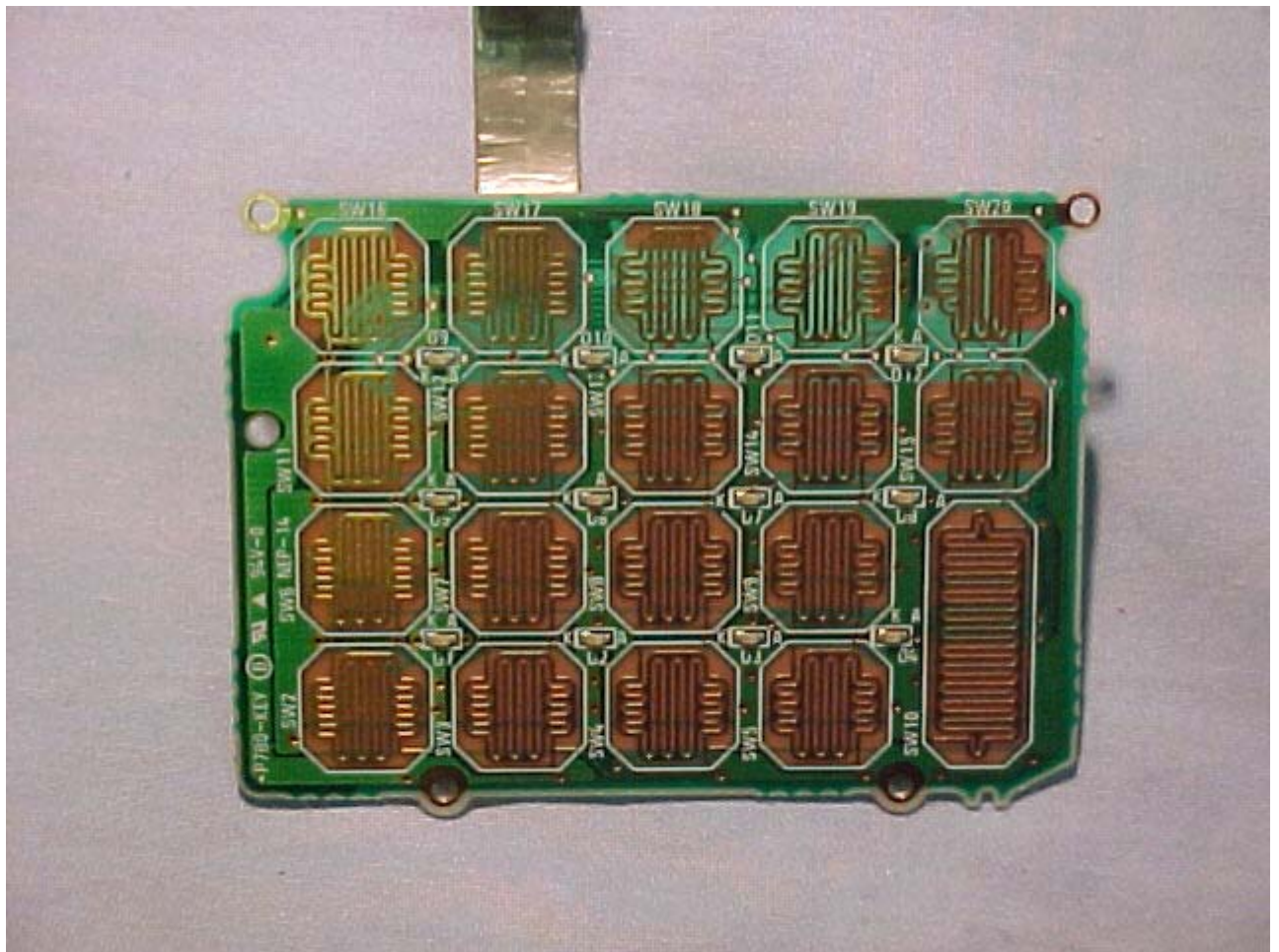
Keyboard Interface underside
