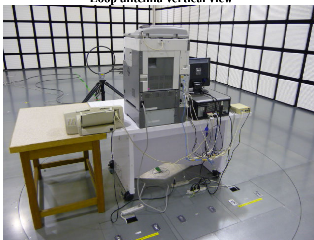
Loop antenna vertical view
