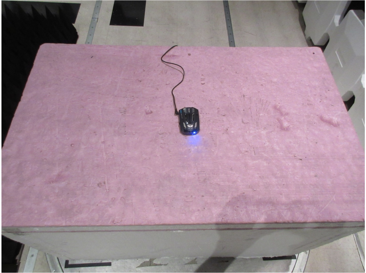
EUT FINAL MEASUREMENT SETUP PHOTO
