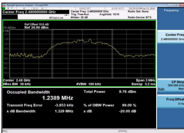
99% Bandwidth: 8DPSK,2480MHz,3DH5
