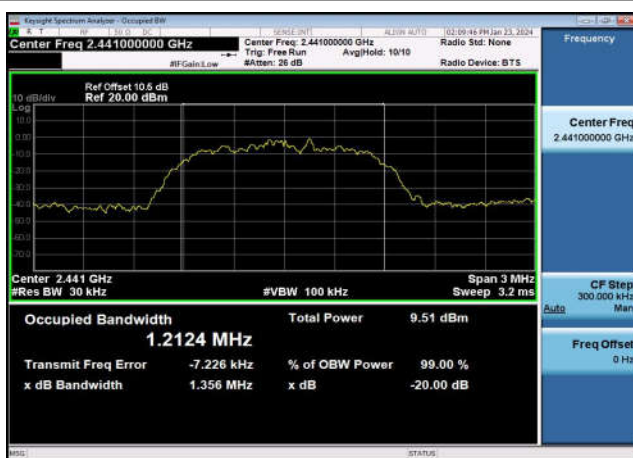
99% Bandwidth: DQPSK,2441MHz,2DH5
