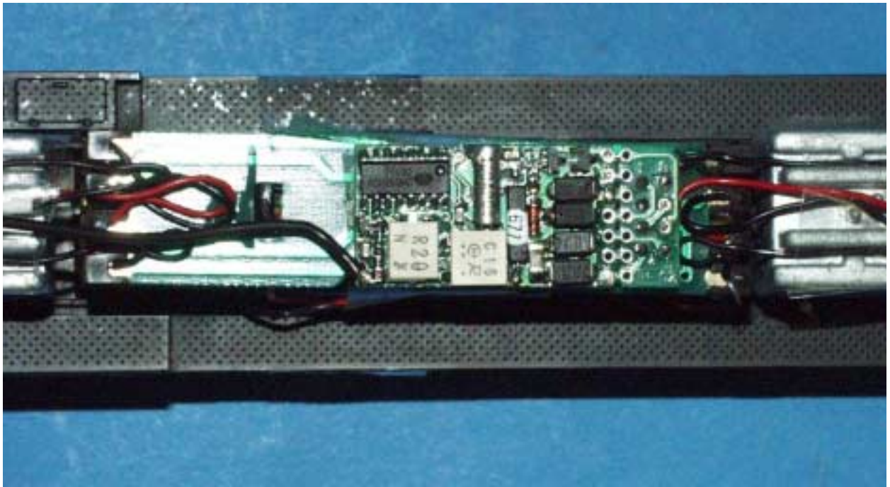
Receiver top detail
