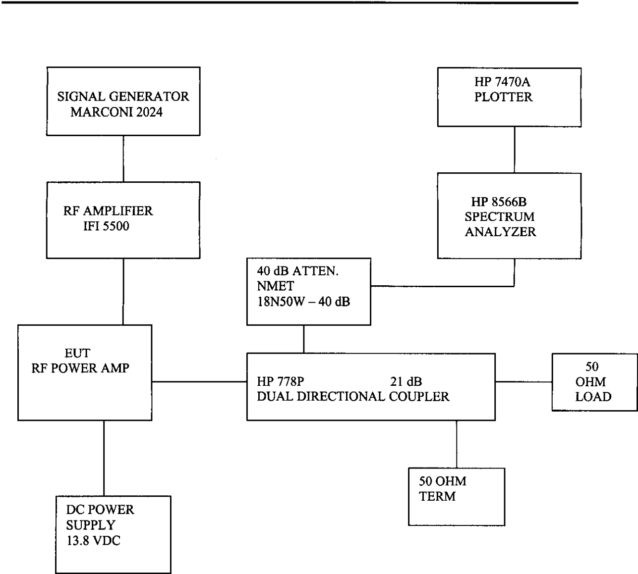
FIGURE 2: Block Diagram (Power Input/Output tests)
