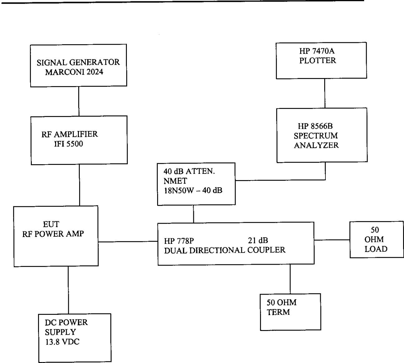
FIGURE 3: Block Diagram (Occupied Bandwidth tests)
