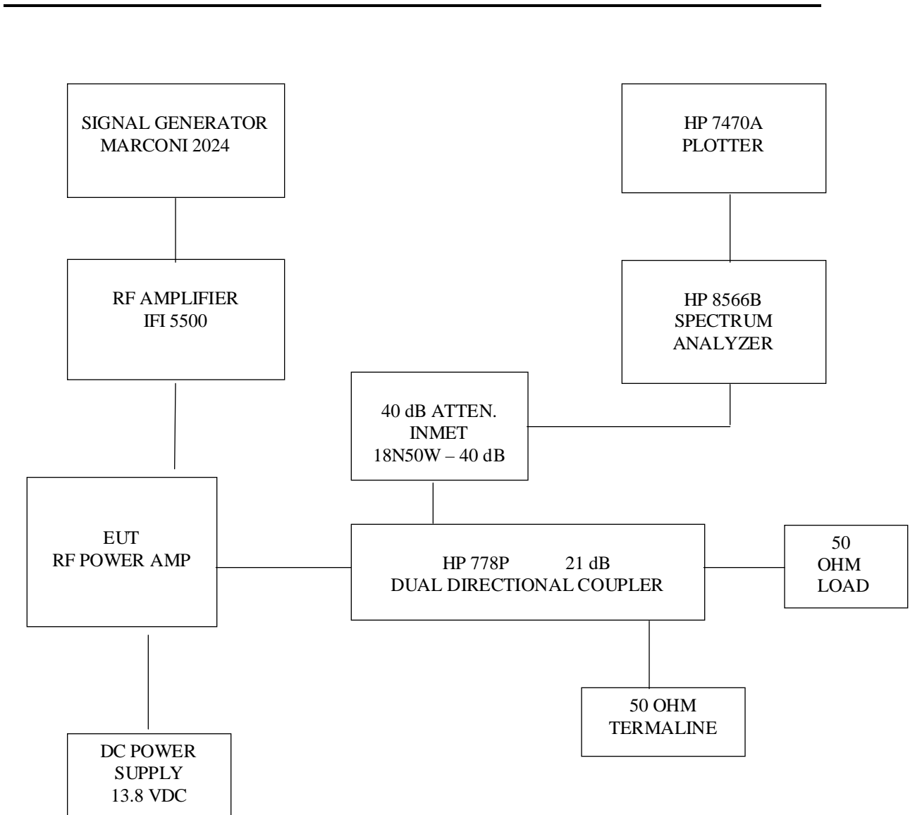
FIGURE 2: Block Diagram (Spurious Emissions tests)
