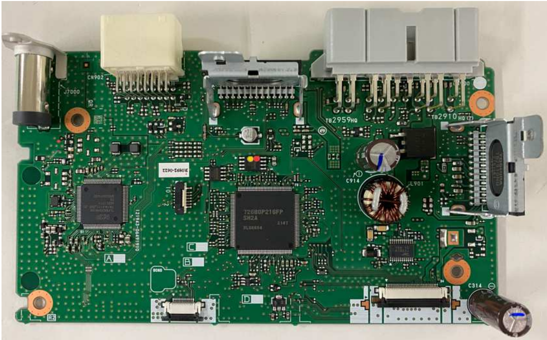
Main PCB
