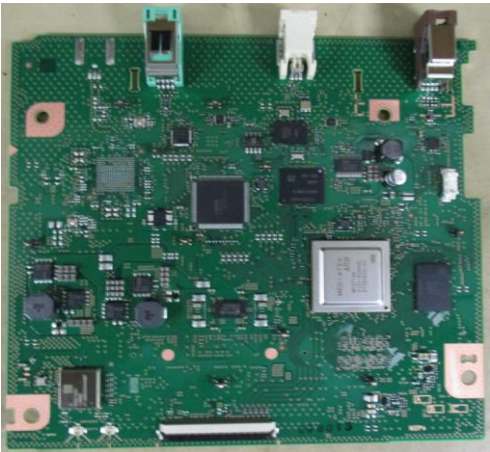
Component side (AUDIO)
