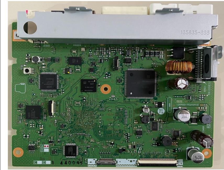
Component side
