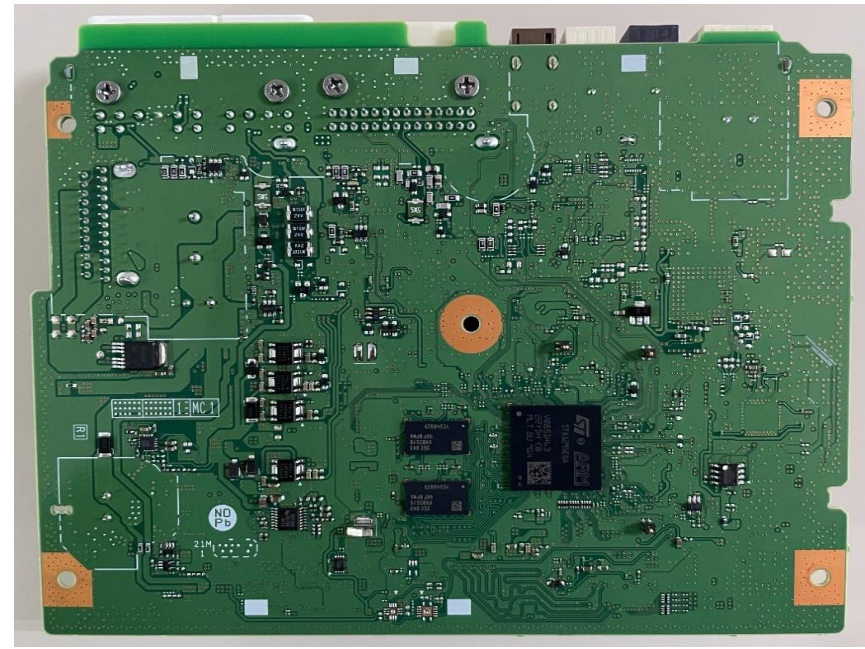
Solder side
