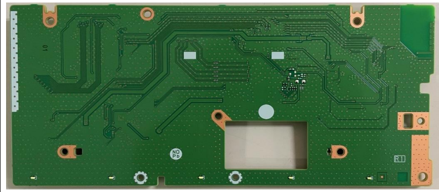
Component side
