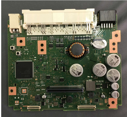
Component side
