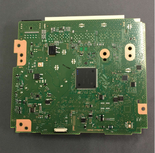
Solder side
