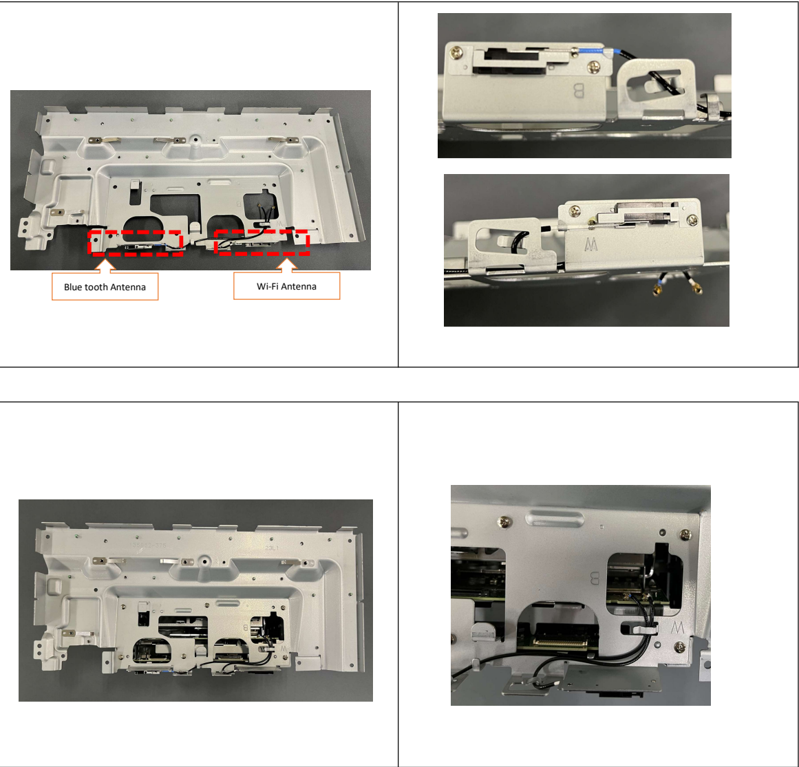
Internal view
