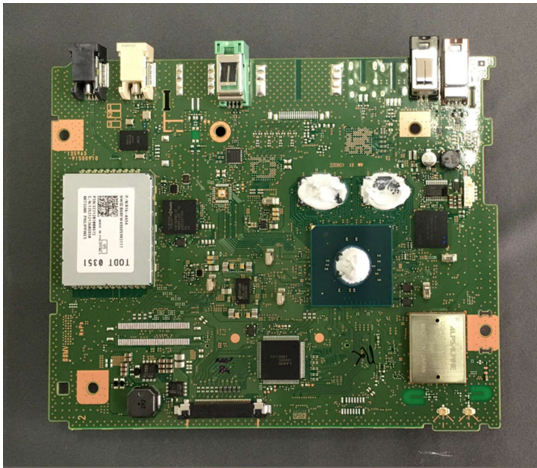
Component side
