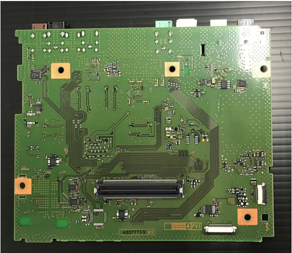
Solder side
