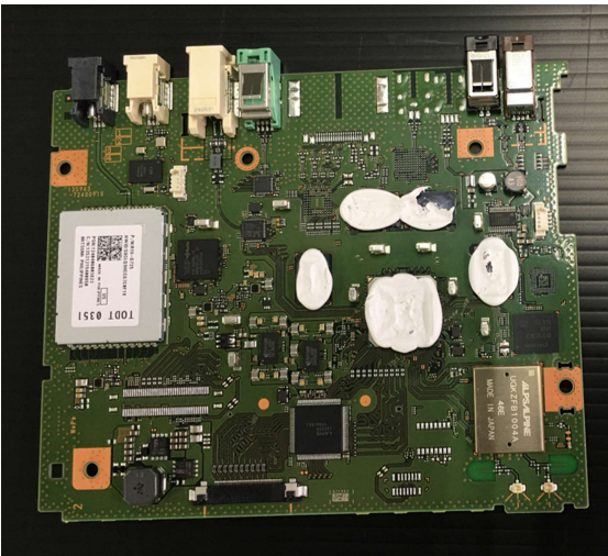
Component side
