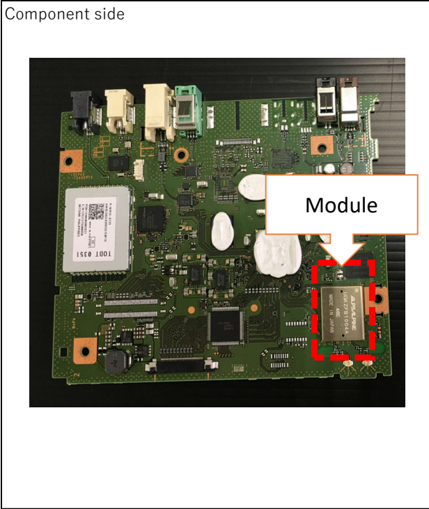
CPU Board
