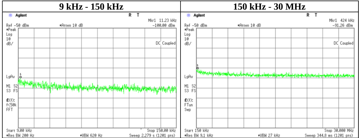
Antenna 1
