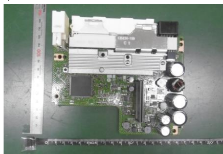
[BT/WiFi ANT , BT/WiFi module mounting position]
