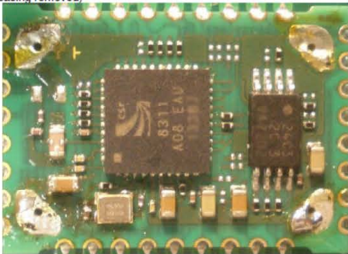
Top View – Internal (Shield casing removed)
