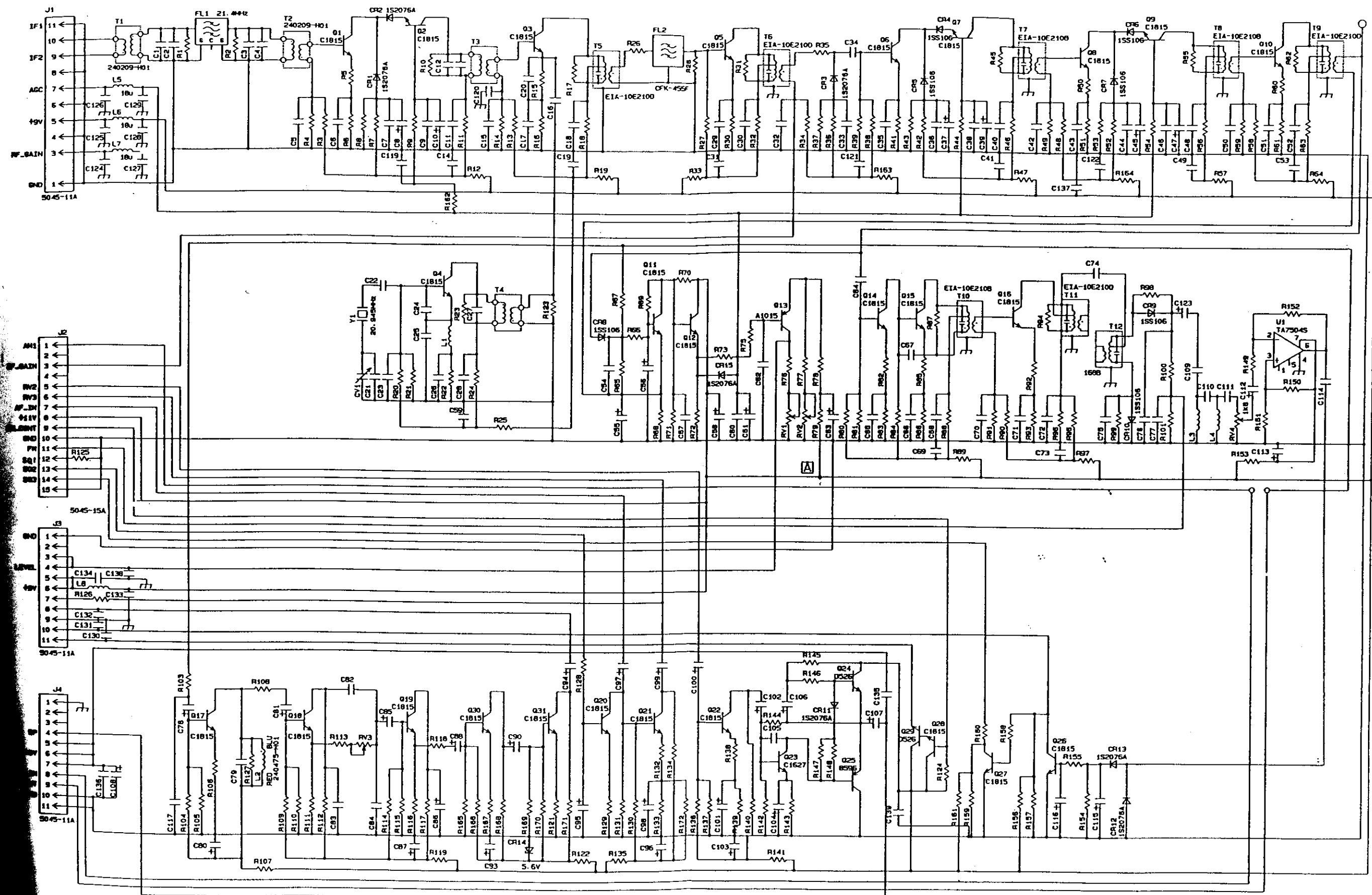
Circuit Diagram of Main Unit PCA IF/AF Drawing No. 322824 TAIYO MUSEN CO., LTD.
