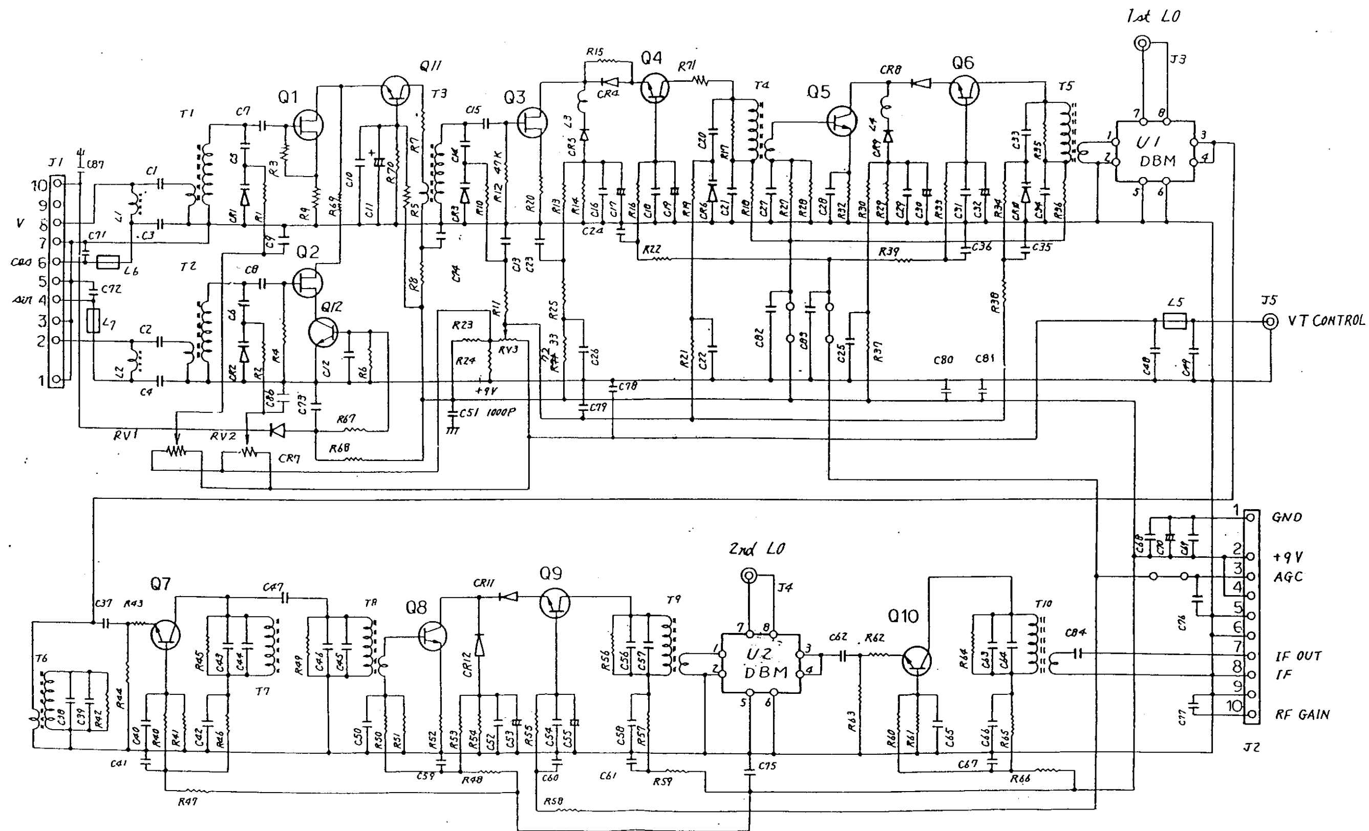
Circuit Diagram of Main Unit PCA HF Drawing No. 332423 TAIYO MUSEN CO., LTD.
