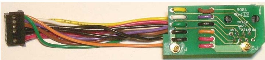
6205 PWB Battery I/O Bd. Bottom
