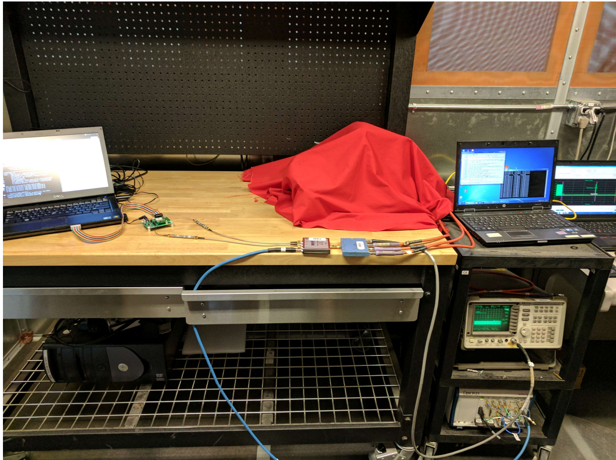
DFS Conducted Test Setup of Client Device
