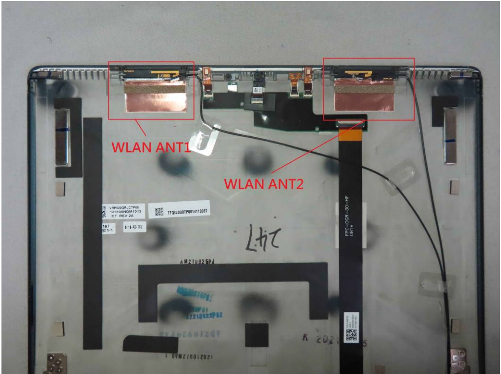
WLAN Antenna
