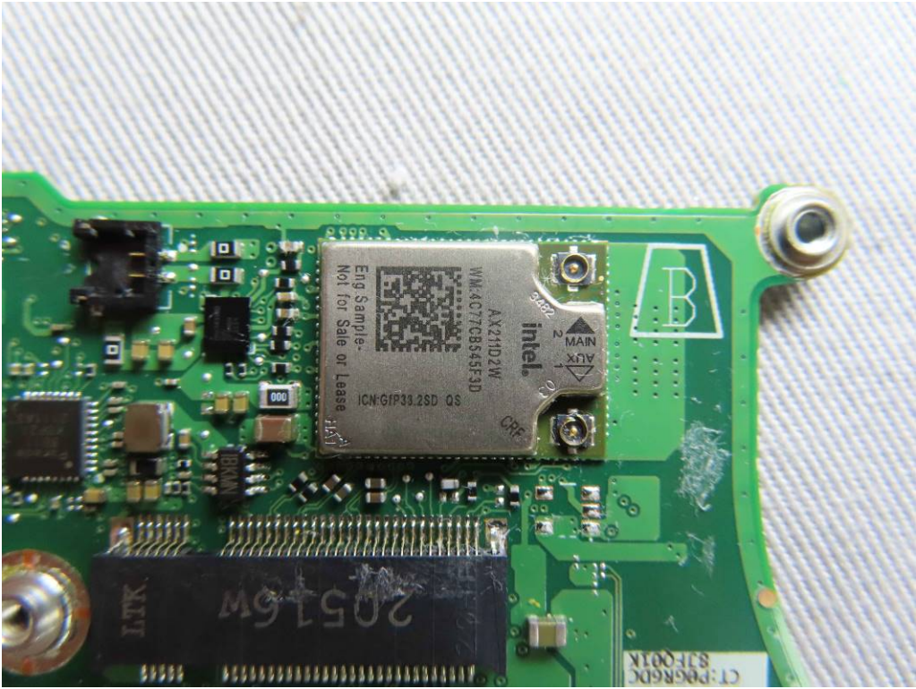
Internal View of EUT – 15
