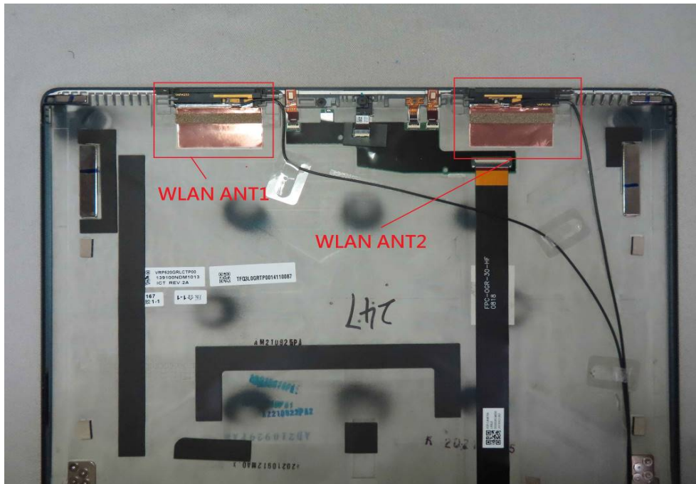
WLAN Antenna
