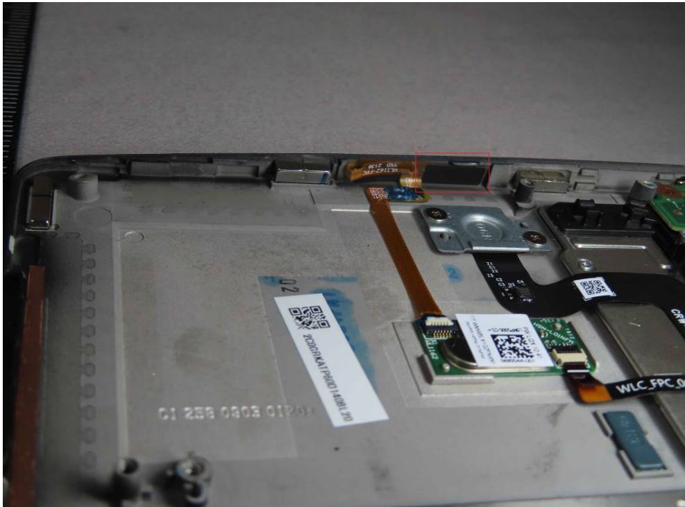
WLAN Antenna
