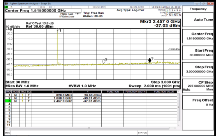
30MHz~3GHz Band26 Part90s 5MHz QPSK 1 0 MidCH26740-819
