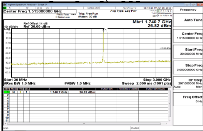
30MHz~3GHz Band66 15MHz QPSK 1 0 MidCH132322-1745
