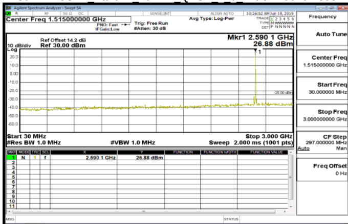
30MHz~3GHz Band41 10MHz QPSK 1 0 MidCH40620-2593
