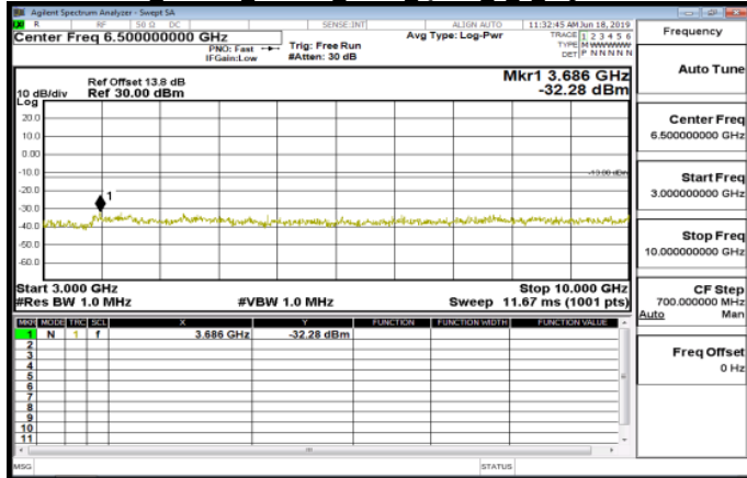
3GHz~10GHz Band26 Part90s 3MHz QPSK 1 0 HighCH26775-822.5
