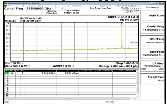
30MHz~3GHz Band38 10MHz QPSK 1 0 HighCH38200-2615
