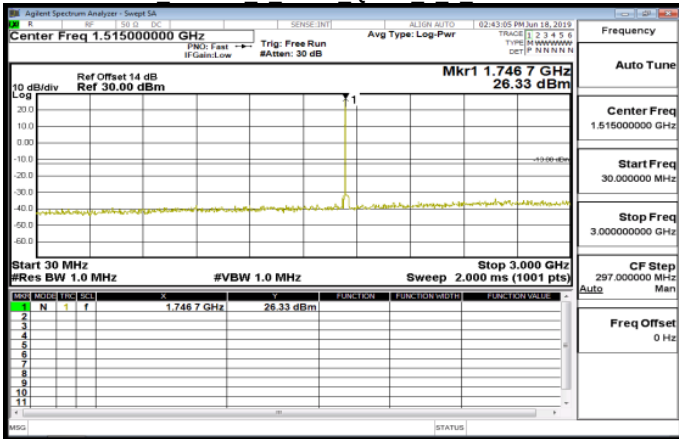
30MHz~3GHz Band66 1 4MHz QPSK 1 0 MidCH132322-1745
