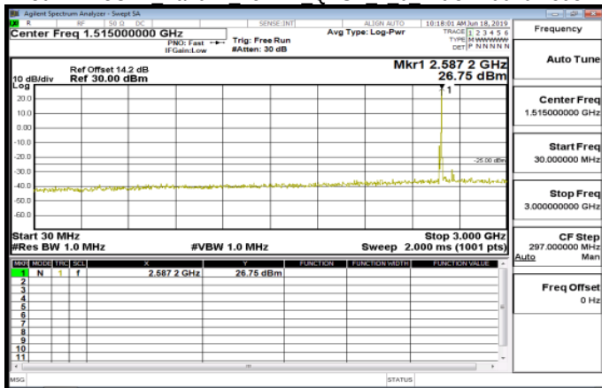
30MHz~3GHz Band41 15MHz QPSK 1 0 MidCH40620-2593
