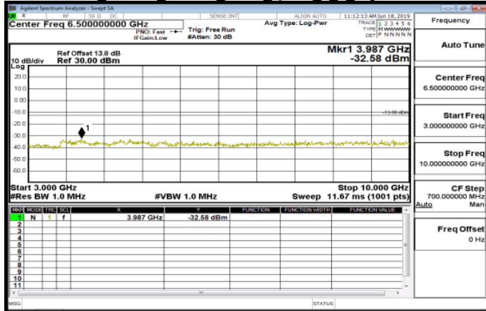
3GHz~10GHz Band26 Part90s 5MHz QPSK 1 0 HighCH26765-821.5
