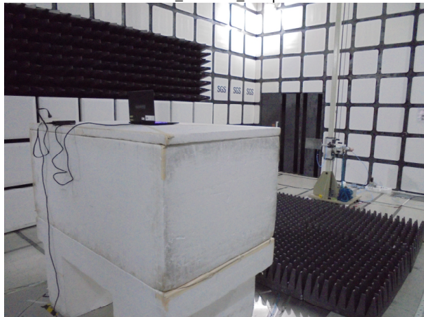
BLE_Radiated_Setup
