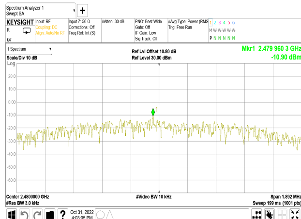
PSD_BLE 2M_HighCH39-2480MHz
