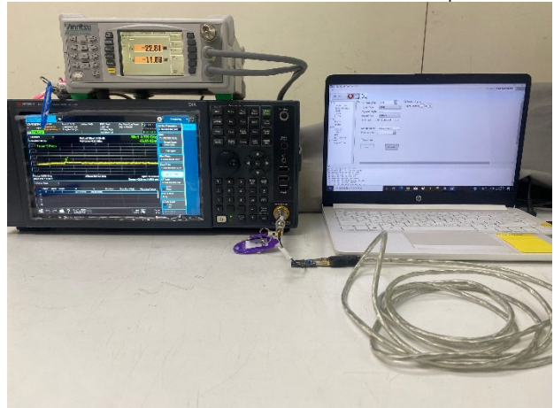
FCC_15_247+ IC_247_BT_Conducted_Setup
