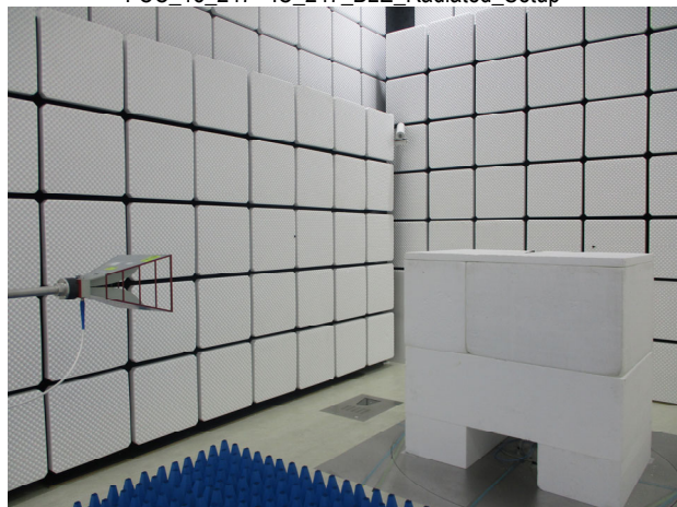
FCC_15_247+ IC_247_BLE_Radiated_Setup
