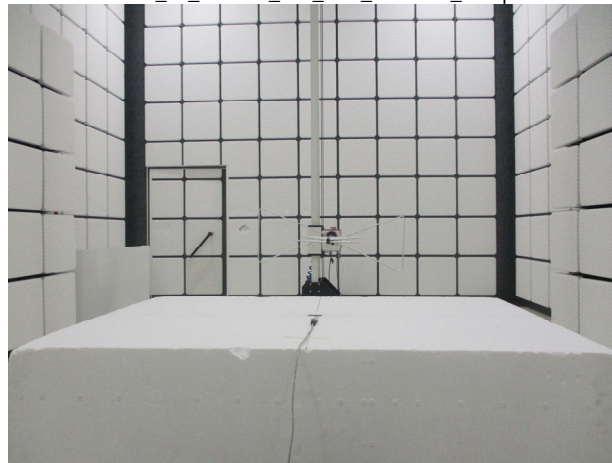
FCC_15_247+ IC_247_BLE_Radiated_Setup
