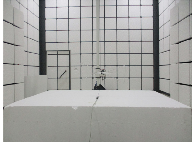
FCC_15_247+ IC_247_BT_Radiated_Setup
