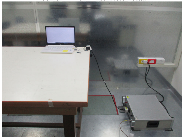
FCC_15_247+ IC_247_Conduction_Setup
