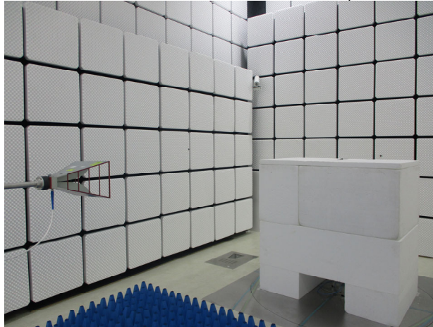
FCC_15_247+ IC_247_BT_Radiated_Setup
