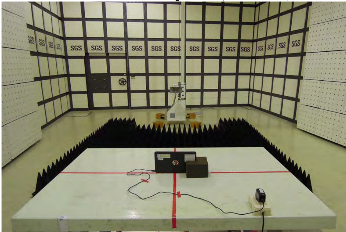
Radiated Emission Set up Photos (Above 1GHz)
