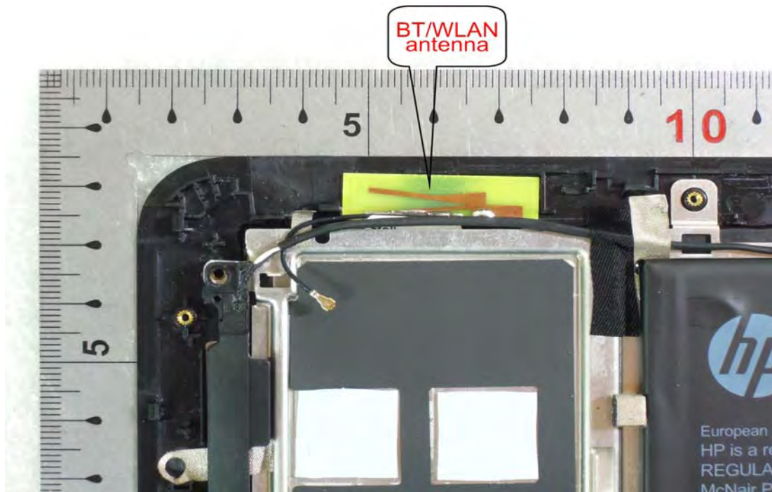
Antenna_ Part No.: 6036B0139101
