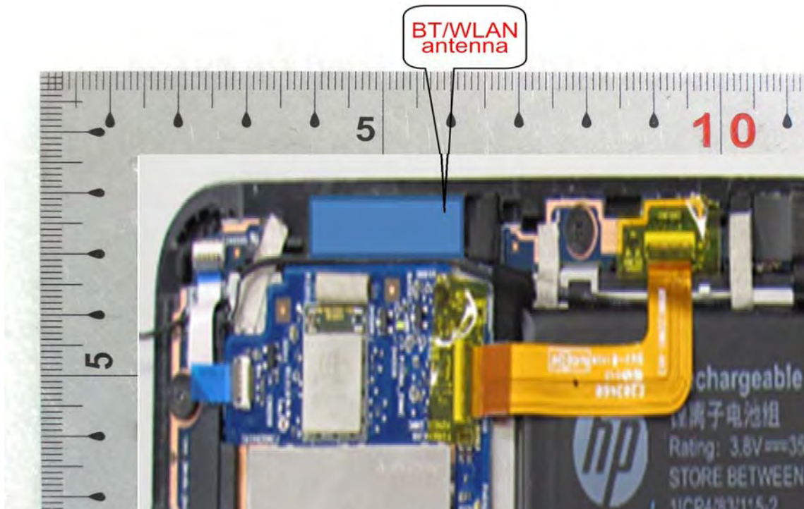
Antenna_ Part No.: 6036B0139201
