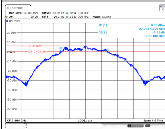
6 dB Bandwidth Plot on Channel 01
