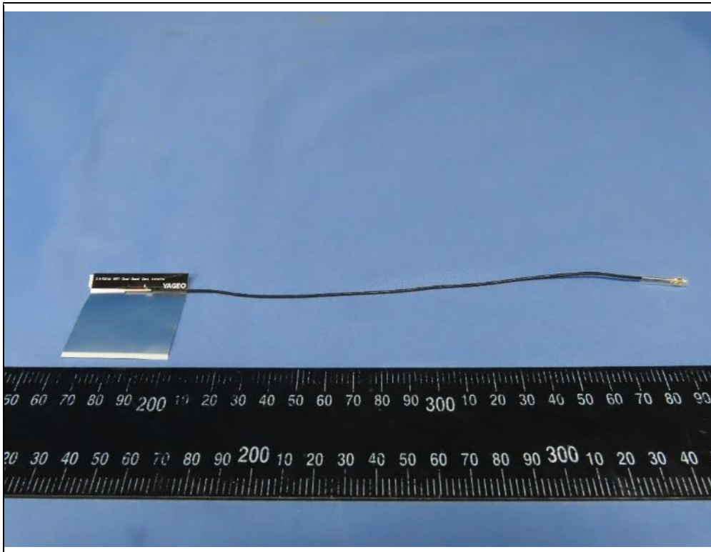
Antenna 3 (Brand: Yageo / Model: ANT-X200P002B24553)
