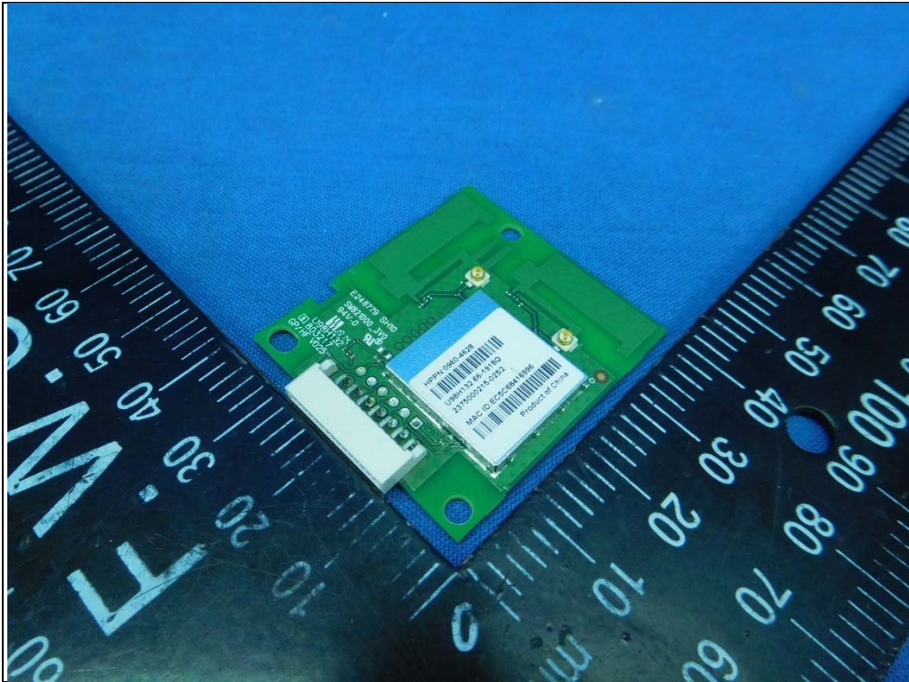
FFC Connector
