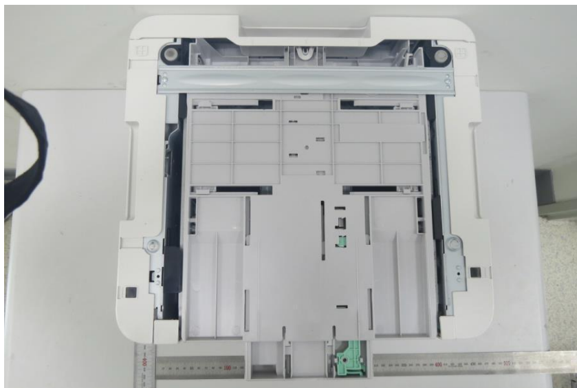
Bottom View
