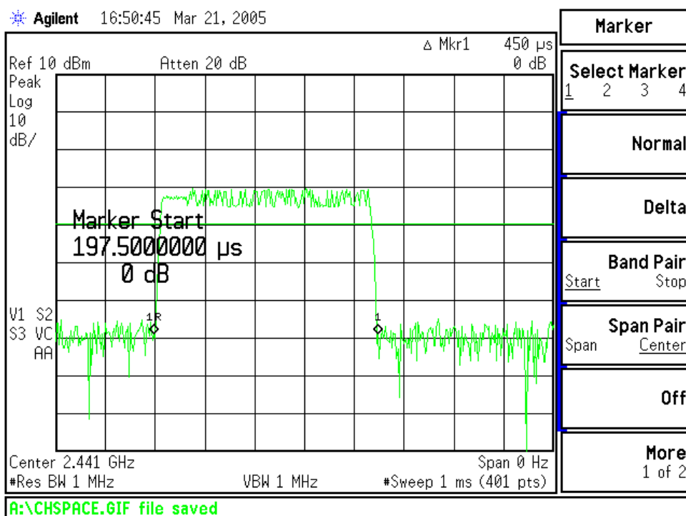
Channel occupancy
