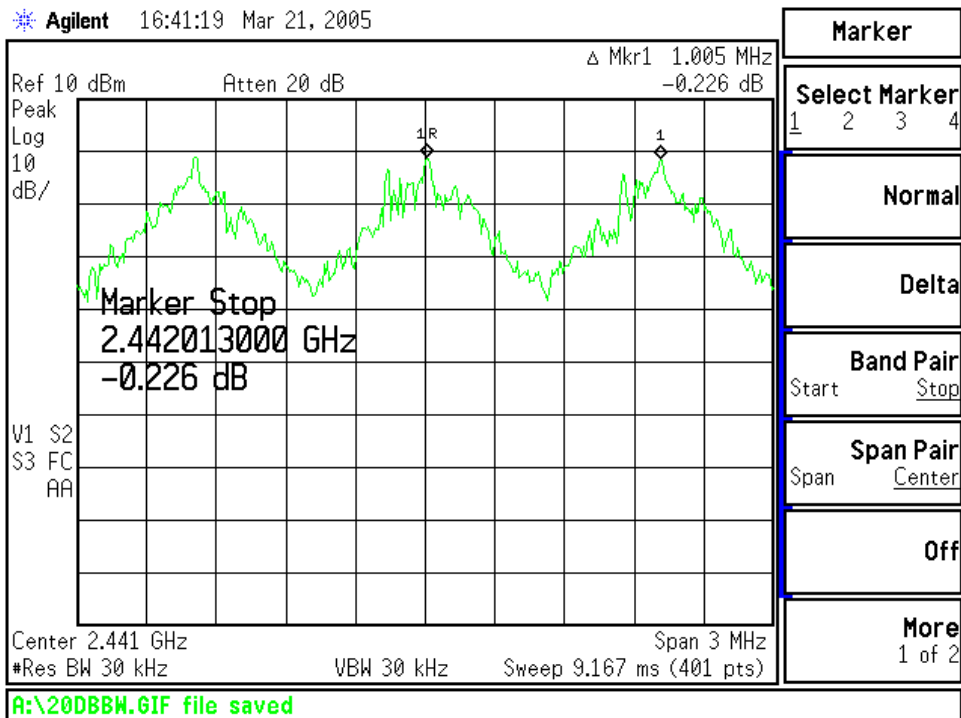
Channel Spacing
